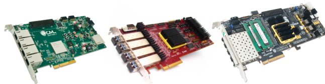
Figure 1: NetFPGA: the enabling platform of OSNT
