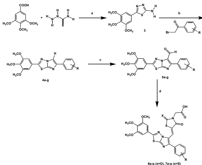
Scheme 1
