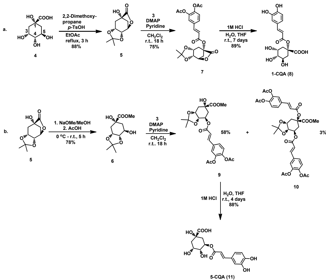
Scheme 2
