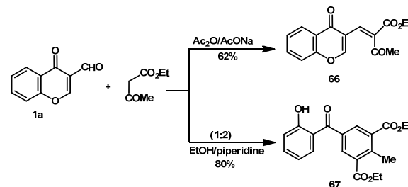
Scheme 31
