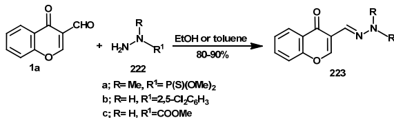
Scheme 104
