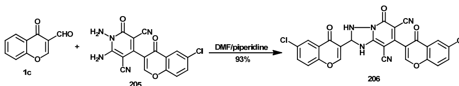
Scheme 96
