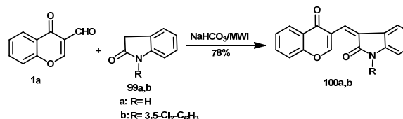
Scheme 49
