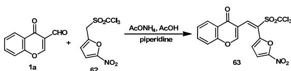
Scheme 29
