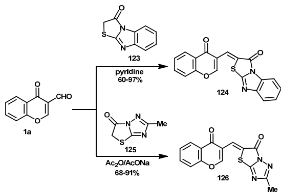
Scheme 60
