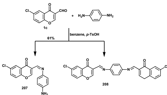
Scheme 97
