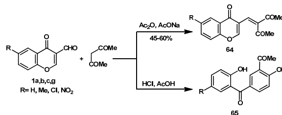
Scheme 30
