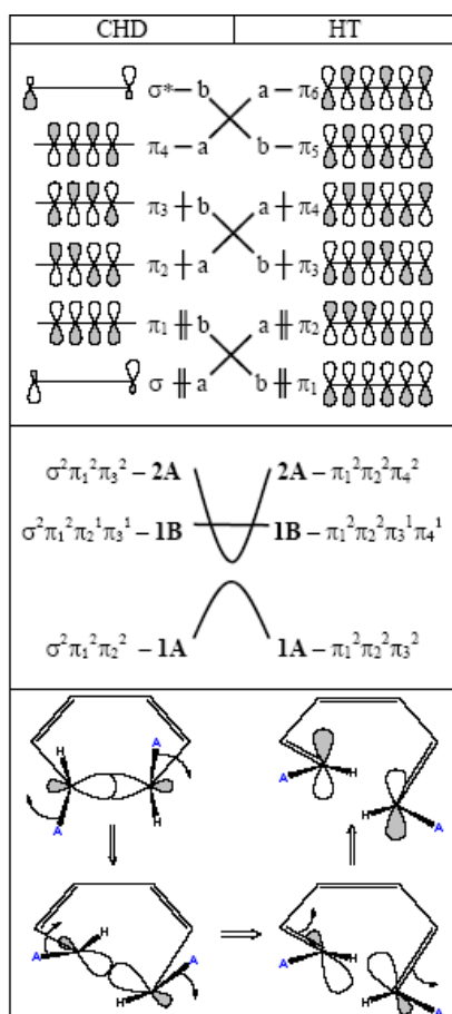
Figure 5. Orbital (top) and state (center) correlation diagrams for photoindated electrocyclic conversion of CHD to HT (bottom). Lines connect the orbitals as they continuously transform along the C_2 -symmetric reaction path. Different orbital occupations give rise to different electronic states. The doubly excited state 2A of CHD correlates with the ground state of HT and vice versa; when their energies approach each other, the states strongly mix and avoid crossing; a true CIX occurs away from symmetric coordinate.
