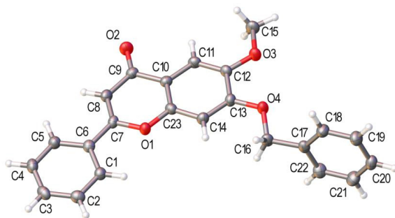
Figure 3. The molecular structure of compound 15 . Displacement ellipsoids are drawn at the 50% probability level.
