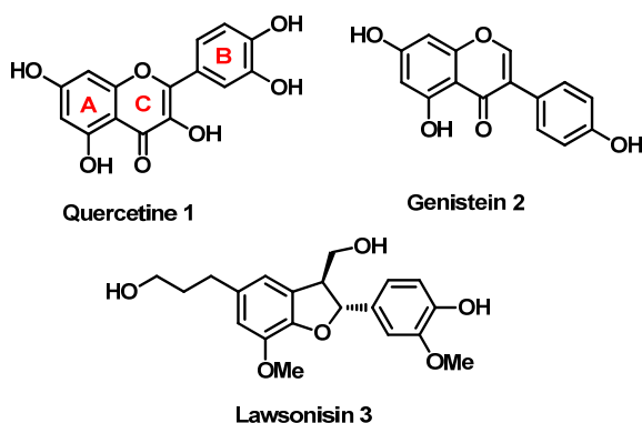
Figure 1. Examples of flavone, isoflavone and benzofuran core containing natural products.
