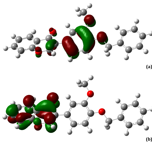
Figure 5. (a) HOMO and (b) LUMO of compound 8 plotted at isovalue of 0.04.
