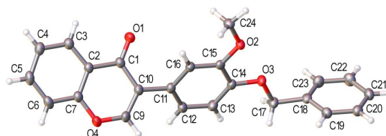
Figure 2. The molecular structure of compound 8 . Displacement ellipsoids are drawn at the 50% probability level.
