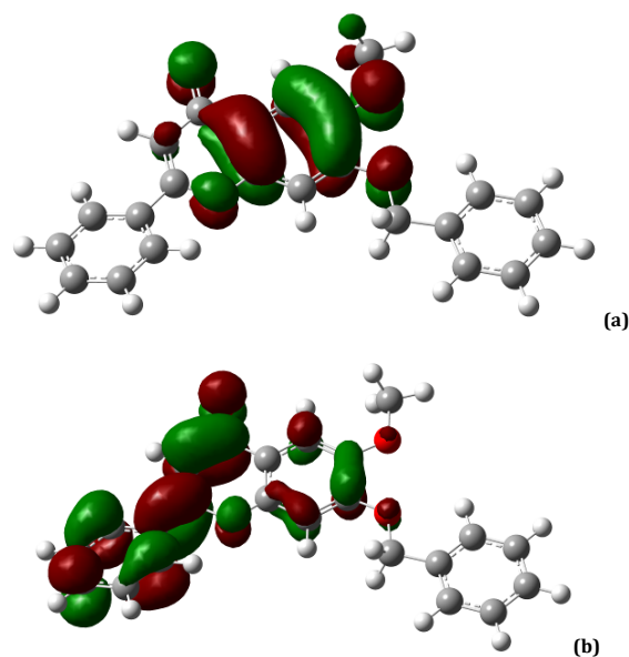
Figure 6. (a) HOMO and (b) LUMO of compound 15 plotted at isovalue of 0.03.
