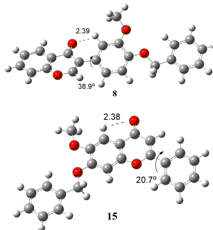
Figure 4. Optimized geometries of compound 8 and 15 at B3LYP/6-311G(d,p). (Bond lengths in Angstrom (Å) and bond angles in degree (°)).
