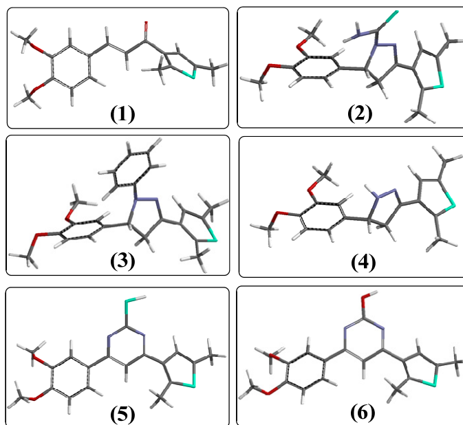
Figure 1. Three dimensional optimized structures 1 to 6 calculated with DFT/B3LYP method.
