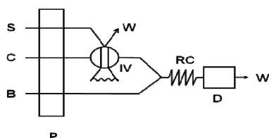
Figure 1. Dynamic manifold used for the discrimination of TRZ: S, sample solution; C, carrier solution; B, buffer solution; P, peristaltic pump; IV, injection valve; RC, reaction coil; D, detector; W, waste.
