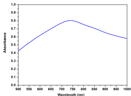
Figure 2. Absorption spectrum of the reduced Folin-Ciocalteu's phenol reagent using 100 \mu g/mL of amlodipine.
