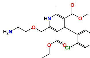
Figure 1. Chemical structure of amlodipine (AMO).
