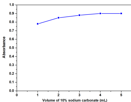
Figure 4. Effect of volume of 10% sodium carbonate on the absorbance of reduced Folin-Ciocalteu's phenol reagent on the absorbance of reduced species at \lambda = 745 nm.
