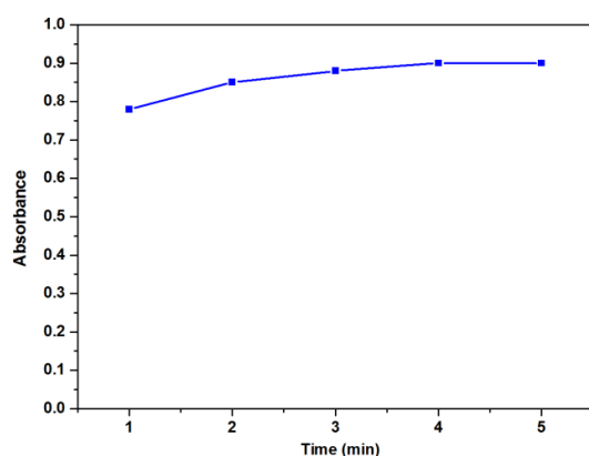
Figure 5. Effect of time on the reduction of Folin-Ciocalteu's phenol reagent on the by amlodipine.
