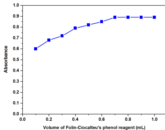
Figure 3. Effect of volume of Folin-Ciocalteu's phenol reagent on the absorbance of reduced species at \lambda = 745 nm.
