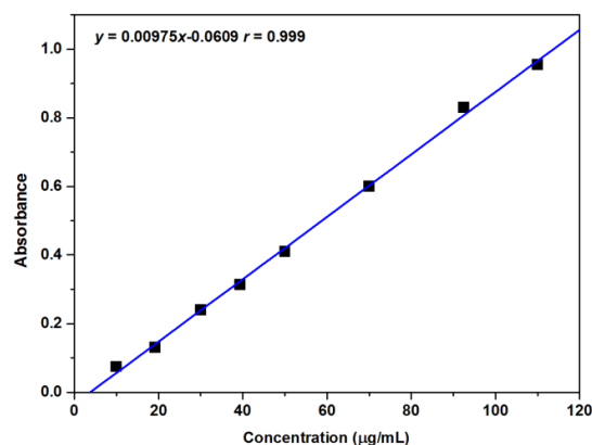
Figure 6. Linearity of the reaction between Folin-Ciocalteu's phenol reagent and amlodipine.
