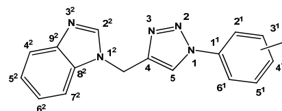
Figure 1. Numbering of carbon atoms in 1,4-disubstituted 1,2,3-triazoles (A-N).
