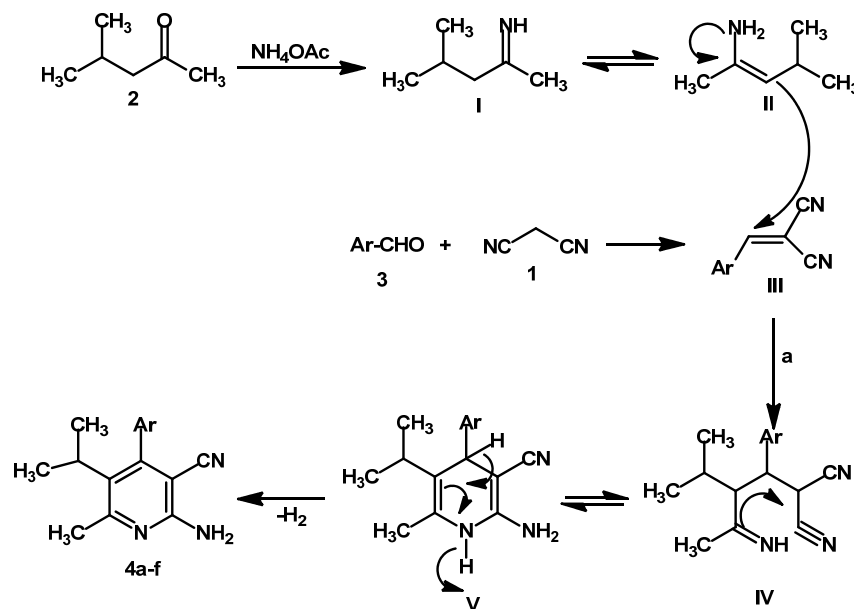
Figure 1. The possible mechanism for synthesis of 2-aminopyridines.
