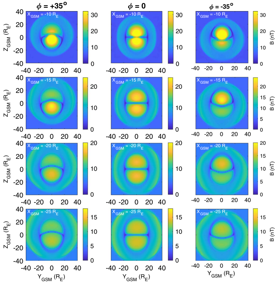
Fig. 12. Cross sections of the tail of the BATSUS model runs showing the magnetic field intensity, B . The rows are for X_{\text{GSM}} (=X_{\text{GSE}}) of (from top to bottom) -10 R_E , -15 R_E , -20 R_E , and -25 R_E . The columns are for dipole tilts \phi of (left) +35^\circ , (middle) 0 and (right) -35^\circ . The outer ring is the bow shock and the two tail lobes, separated by the low-field plasma sheet can be clearly seen. At all X_{\text{GSM}} , the field in the “winter” lobe (south for \phi = +35^\circ , north for \phi = -35^\circ ) is similar to that for the \phi = 0 case (and sometimes very slightly enhanced), whereas for the “summer” lobe (north for \phi = +35^\circ , south for \phi = -35^\circ ) it is always considerably lower.
