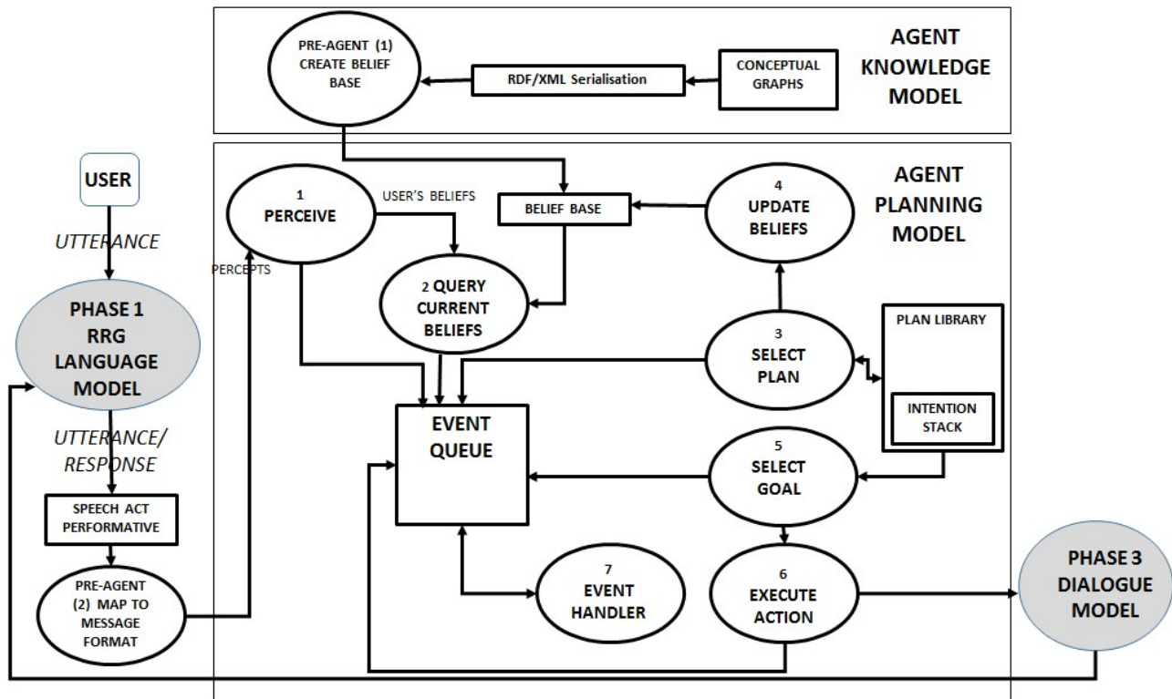
FIGURE 4. DESIGN FRAMEWORK - AGENT COGNITIVE MODEL (PANESAR, 2017).
