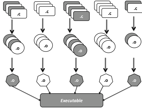
Figure 1: An Example Code Base . From the top: each source file creates a corresponding object file; multiple object files are combined into intermediate compilation units (CU); and multiple CUs are merged to form the executable. All shaded blocks indicate modified files.
