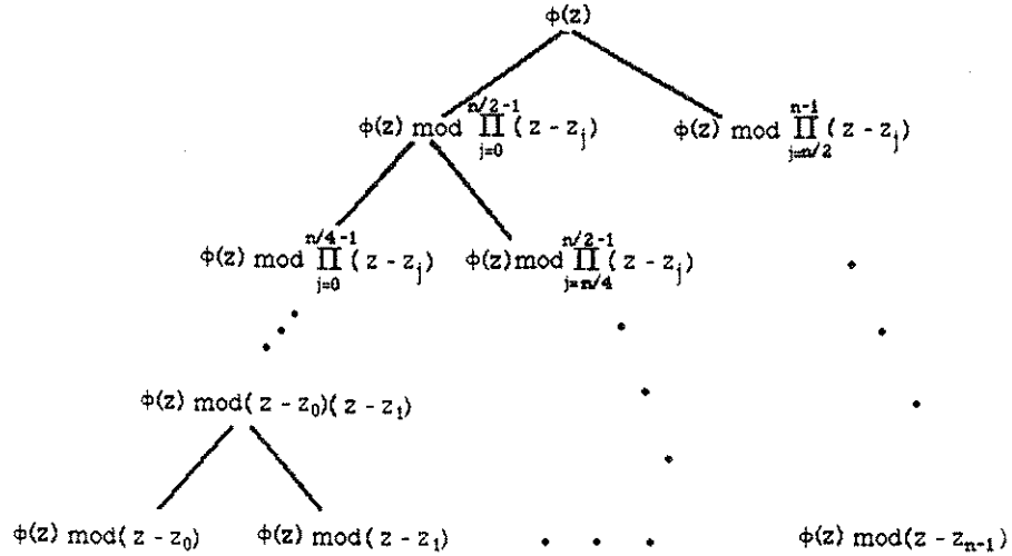
Figure 1. Tree for evaluating a polynomial \phi(z) at n = 2^k points. Note that it has k = \log n levels.
