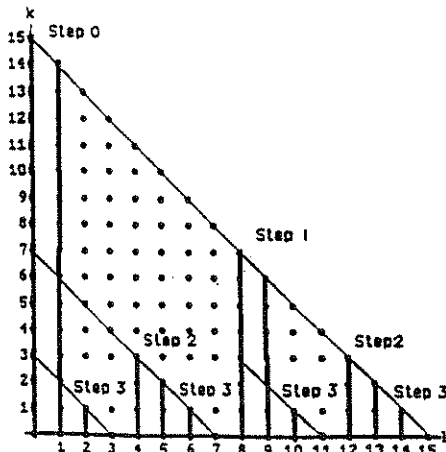
Figure 3. Computation of the Z_l(0) for l < n by a cascade of convolutions of of decreasing size. The relevant ranges of Z are highlighted, and the step in which they are calculated is indicated.
