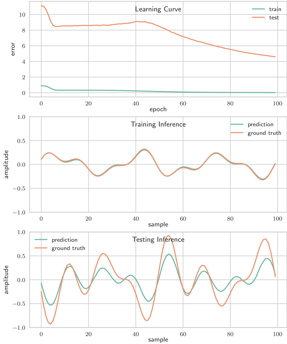
Figure 3.8: Model using regular complex inputs, regular complex outputs, and sigmoidal activation on the real and imaginary components. Top: learning curves on the training and testing sets. Middle: inference on a random example from the training set. Bottom: inference on a random example from the testing set.
