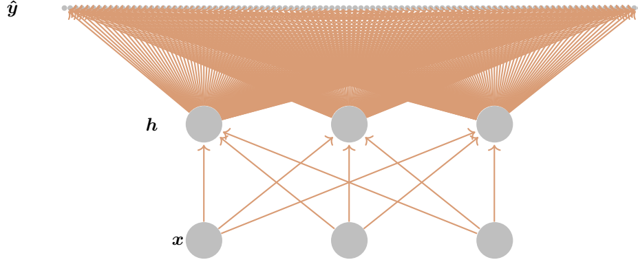
Figure 3.6: Basic model architecture showing D = 3 input and hidden nodes, with N = 100 output nodes.
