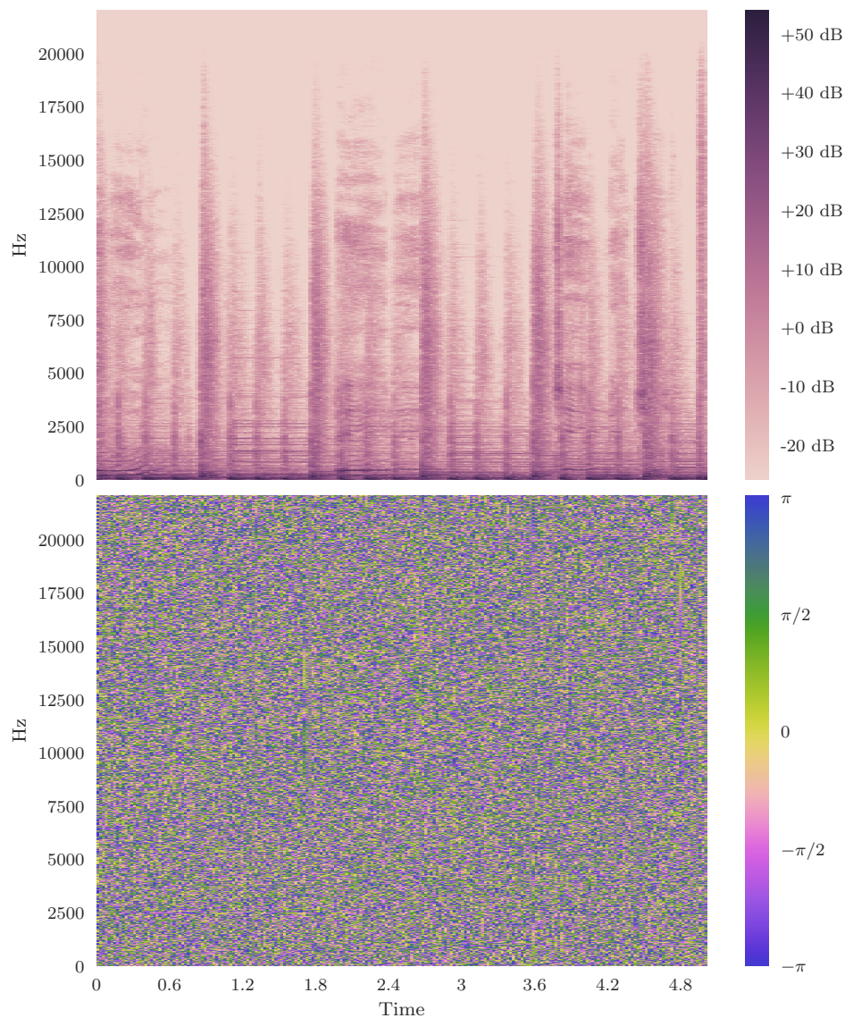
Figure 2.2: STFT corresponding to a few seconds of the pop music recording depicted in Fig. 2.1. Top: power spectrogram, in decibels. Harmonics, seen as horizontal bands of energy are apparent in the lower frequencies. Transient sounds, such as drum hits, are represented by bursts of energy across all frequencies. Bottom: phase spectrogram, in radians. It is difficult to visually parse patterns from the phase spectra.
