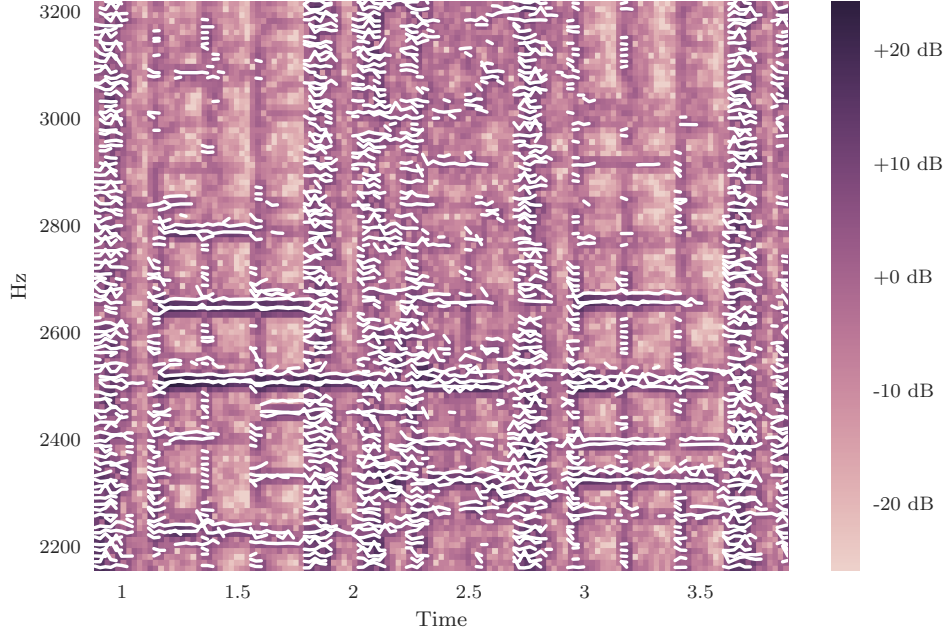
Figure 2.3: Zoomed-in power portion of spectrogram shown in Fig. 2.2. Bins having at least 0 dB energy are overlaid with phase-based frequency estimations (in white). With a small amount of processing, the phase spectra reveal an estimate of the true frequency that each bin’s energy is associated with, information which is unavailable in the magnitude spectra.
