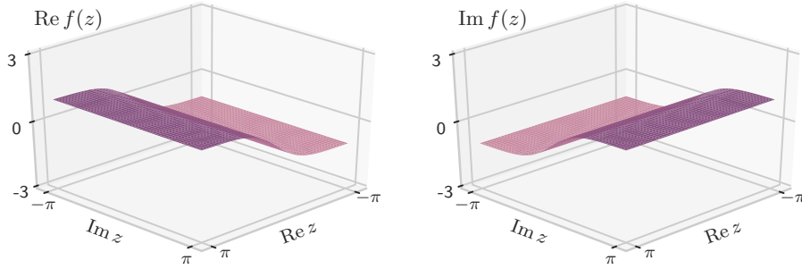
Figure 3.2: Surface plots for the real and imaginary parts of the split real-imaginary hyperbolic tangent function.
