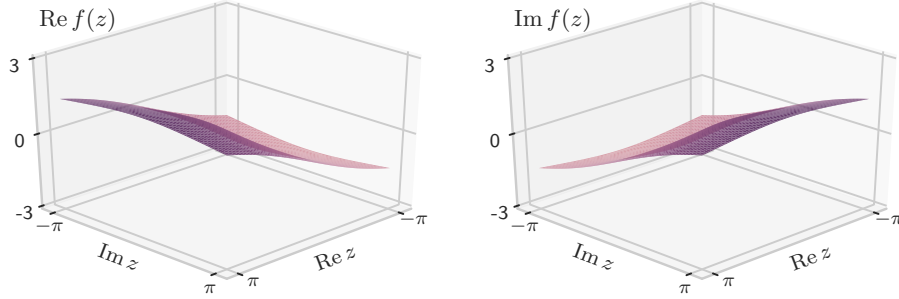
Figure 3.3: Surface plots for the real and imaginary parts of the split phase-preserving function proposed by (Georgiou & Koutsougeras, 1992).
