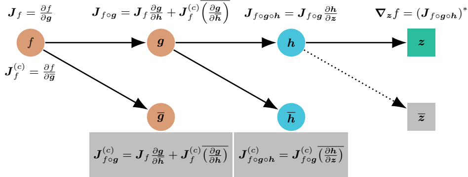
Figure 3.4: Computational dependency graph for a composition of holomorphic and non-holomorphic functions. Tan circular nodes: non-holomorphic functions. Blue circular nodes: holomorphic functions. Rectangular nodes: inputs. The non-holomorphic functions are dependent on their inputs and the conjugate of their inputs. The holomorphic functions are necessarily not dependent on the conjugate of their inputs.
