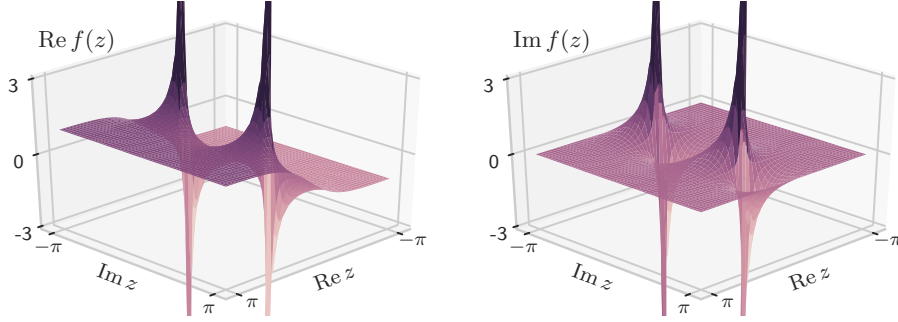
Figure 3.1: Surface plots for the real and imaginary parts of the hyperbolic tangent function.
