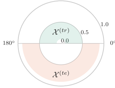
Figure 3.7: Non-overlapping training and testing data, shown in polar coordinates.
