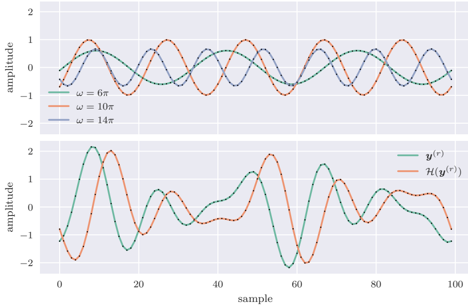
Figure 3.5: Top: three real sinusoids corresponding to arbitrary vectors \alpha and \varphi . Bottom: corresponding real-valued output \mathbf{f}(\alpha, \varphi) and the Hilbert transform of \mathbf{f} . Black markers indicate sample points corresponding to \mathbf{t} .
