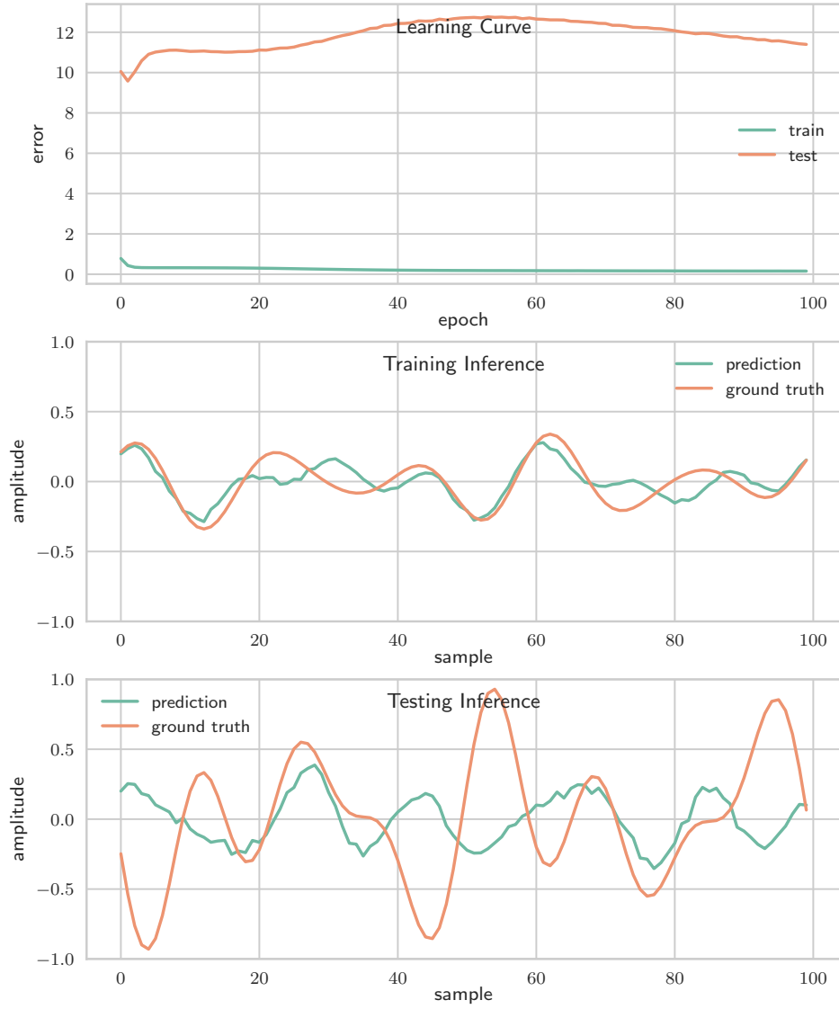
Figure 3.9: Model using real amplitude-phase inputs, regular real outputs, and sigmoidal activations. Top: learning curves on the training and testing sets. Middle: inference on a random example from the training set. Bottom: inference on a random example from the testing set.
