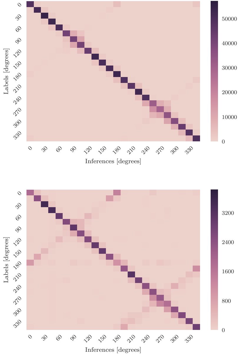
Figure 4.3: Confusion matrices. Top: best complex model. Bottom: baseline complex model using features proposed in (Tsuzuki, Kugler, Kuroyanagi, & Iwata, 2013).
