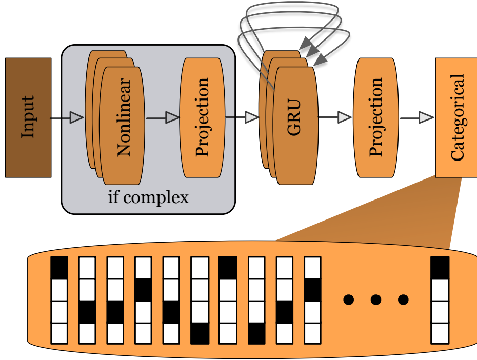
Figure 5.2: DSE Encoder model.
