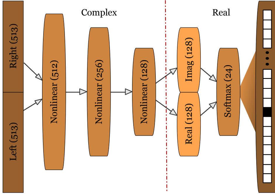
Figure 4.2: Architecture of the binaural source localization model. Numbers in parentheses indicate number of units. The left and right frequency-domain inputs are fed into three complex nonlinear layers. The real and imaginary parts of the third layer are concatenated into a real vector, which is followed by a final nonlinear layer with a softmax activation.
