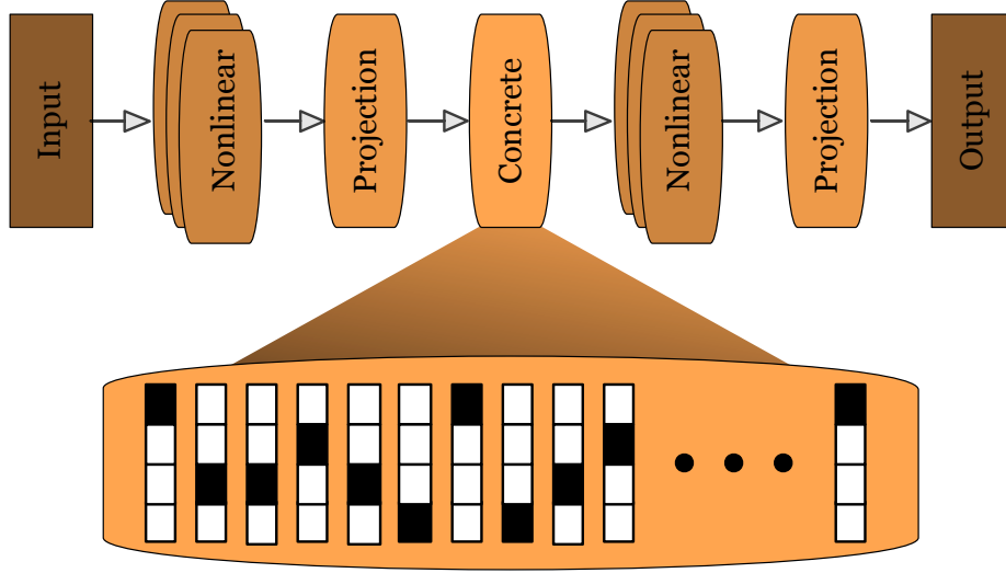
Figure 5.1: Conditional VQ model.
