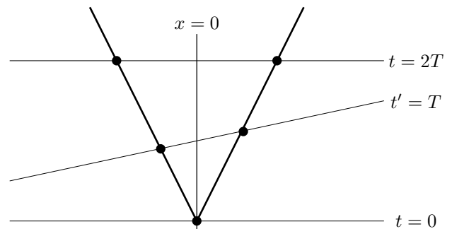
Figure 5. The reported effect disappears if one first evolves the system to an hypersurface of constant t' and then back into an hypersurface of constant t .
