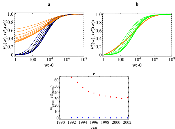
FIG. 1: (Color online) Edge weights in the weighted undirected ITN. a ) cumulative distributions of edge weights, for all years from 1992 (top) to 2002 (bottom). Orange (upper curves): real network; blue (lower curves): expectation for the maximum-entropy null model with specified strengths. b ) same as the previous panel, but excluding zero weights (missing links). Orange (dark grey): real network; green (light grey): null model. c ) percentage of missing links as a function of time. Red (upper points): real network; blue (lower points): null model.
