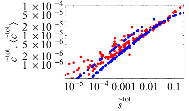
FIG. 11: (Color online) Total weighted clustering coefficient \tilde{c}_i^{\text{tot}} versus total strength \tilde{s}_i^{\text{tot}} in the 2002 snapshot of the real weighted directed ITN (red, lighter points), and corresponding average over the null model with specified out-strengths and in-strengths (blue, darker points).
