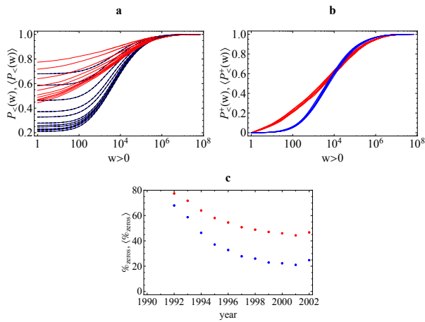
FIG. 8: (Color online) Edge weights in the weighted directed ITN. Red (light grey, upper curves/points): real network; blue (dark grey, lower curves/points): expectation for the maximum-entropy ensemble with specified out-strengths and in-strengths. a ) cumulative distributions of edge weights in all years from 1992 (top) to 2002 (bottom). b ) same as the previous panel, but excluding zero weights (missing links). c ) percentage of missing links as a function of time.
