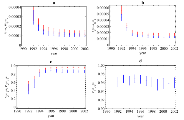
FIG. 15: (Color online) Temporal evolution of the properties of the (rescaled) total weighted clustering coefficient \tilde{c}_i^{tot} in the 1992-2002 snapshots of the real weighted directed ITN and of the corresponding null model with specified out-strengths and in-strengths. a) average of \tilde{c}_i^{tot} across all vertices (red, upper symbols: real data; blue, lower symbols: null model). b) standard deviation of \tilde{c}_i^{tot} across all vertices (red, upper symbols: real data; blue, lower symbols: null model). c) correlation coefficient between \tilde{c}_i^{tot} and \tilde{s}_i^{tot} (red, upper symbols: real data; blue, lower symbols: null model). d) correlation coefficient between \tilde{c}_i^{tot} and \langle \tilde{c}_i^{tot} \rangle . The 95% confidence intervals of all quantities are represented as vertical bars.
