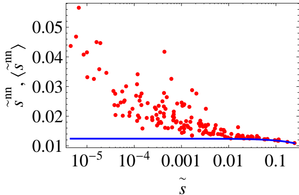
FIG. 2: (Color online) Average nearest neighbor strength \langle \tilde{s}^{nn} \rangle versus strength \tilde{s}_i in the 2002 snapshot of the real weighted undirected ITN (red points), and corresponding average over the maximum-entropy ensemble with specified strengths (blue solid curve).
