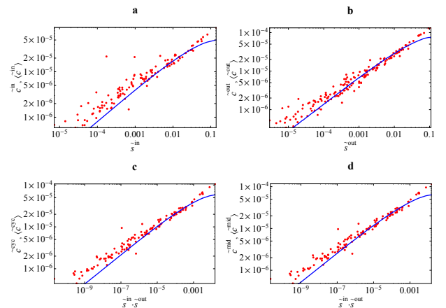
FIG. 12: (Color online) Weighted clustering coefficients versus vertex strengths in the 2002 snapshot of the real weighted directed ITN (red points), and corresponding averages over the null model with specified out-strengths and in-strengths (blue solid curves). a) \tilde{c}_i^{\text{in}} versus \tilde{s}_i^{\text{in}} ; b) \tilde{c}_i^{\text{out}} versus \tilde{s}_i^{\text{out}} ; c) \tilde{c}_i^{\text{cyc}} versus \tilde{s}_i^{\text{in}} \cdot \tilde{s}_i^{\text{out}} ; d) \tilde{c}_i^{\text{mid}} versus \tilde{s}_i^{\text{in}} \cdot \tilde{s}_i^{\text{out}} .
