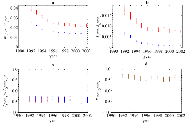
FIG. 13: (Color online) Temporal evolution of the properties of the (rescaled) total average nearest neighbor strength \tilde{s}_i^{tot/tot} in the 1992-2002 snapshots of the real weighted directed ITN and of the corresponding null model with specified out-strengths and in-strengths. a) average of \tilde{s}_i^{tot/tot} across all vertices (red, upper symbols: real data; blue, lower symbols: null model). b) standard deviation of \tilde{s}_i^{tot/tot} across all vertices (red, upper symbols: real data; blue, lower symbols: null model). c) correlation coefficient between \tilde{s}_i^{tot/tot} and \tilde{s}_i^{tot/tot} (red: real data; blue: null model, indistinguishable from real data). d) correlation coefficient between \tilde{s}_i^{tot/tot} and \langle \tilde{s}_i^{tot/tot} \rangle . Vertical bars are 95% confidence intervals.
