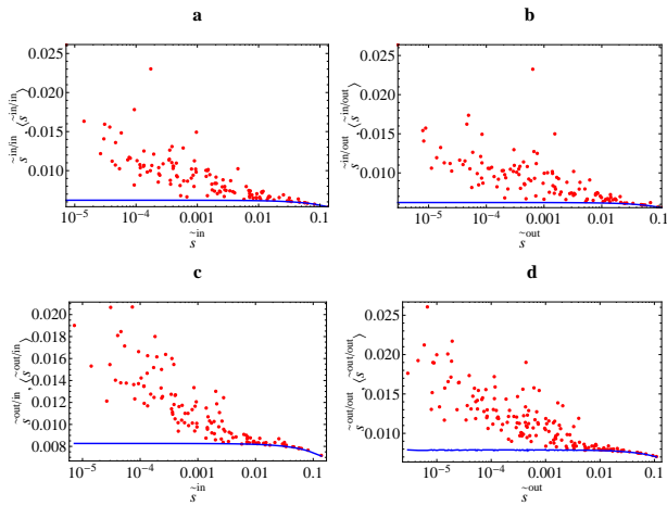
FIG. 10: (Color online) Directed average nearest neighbor strengths versus vertex strengths in the 2002 snapshot of the real weighted directed ITN (red points), and corresponding averages over the null model with specified out-strengths and in-strengths (blue solid curves). a) \tilde{s}_i^{\text{in}/\text{in}} versus \tilde{s}_i^{\text{in}} ; b) \tilde{s}_i^{\text{in}/\text{out}} versus \tilde{s}_i^{\text{in}} ; c) \tilde{s}_i^{\text{out}/\text{in}} versus \tilde{s}_i^{\text{out}} ; d) \tilde{s}_i^{\text{out}/\text{out}} versus \tilde{s}_i^{\text{out}} .
