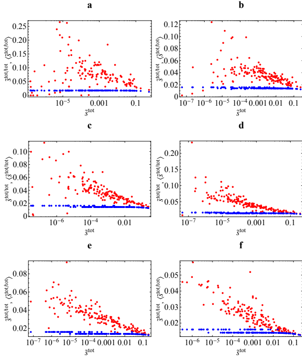
FIG. 17: (Color online) Total average nearest neighbor strength \tilde{s}_i^{tot/tot} versus total strength \tilde{s}_i^{tot} in the 2002 snapshots of the commodity-specific (disaggregated) versions of the real weighted directed ITN (red, upper points), and corresponding average over the maximum-entropy ensemble with specified out-strengths and in-strengths (blue, lower points). a) commodity 93; b) commodity 09; c) commodity 39; d) commodity 90; e) commodity 84; f) aggregation of the top 14 commodities (see Ref. [1] for details). From a) to f), the intensity of trade and level of aggregation increases.
