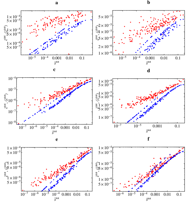
FIG. 18: (Color online) Total weighted clustering coefficient \tilde{c}_i^{tot} versus total strength \tilde{s}_i^{tot} in the 2002 snapshots of the commodity-specific (disaggregated) versions of the real weighted directed ITN (red, upper points), and corresponding average over the maximum-entropy ensemble with specified out-strengths and in-strengths (blue, lower points). a) commodity 93; b) commodity 09; c) commodity 39; d) commodity 90; e) commodity 84; f) aggregation of the top 14 commodities (see Ref. [1] for details). From a) to f), the intensity of trade and level of aggregation increases.
