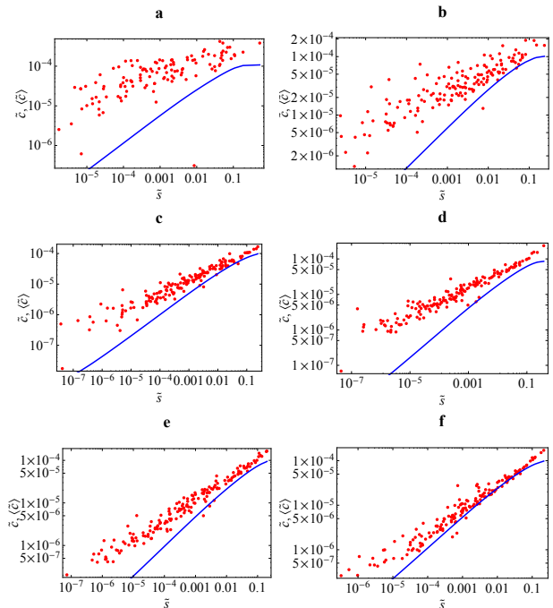
FIG. 7: (Color online) Weighted clustering coefficient \tilde{c}_i versus strength \bar{s}_i in the 2002 snapshots of the commodity-specific (disaggregated) versions of the real weighted undirected ITN (red points), and corresponding average over the maximum-entropy ensemble with specified strengths (blue solid curves). a) commodity 93; b) commodity 09; c) commodity 39; d) commodity 90; e) commodity 84; f) aggregation of the top 14 commodities (see Ref. [1] for details). From a) to f), the intensity of trade and level of aggregation increases.
