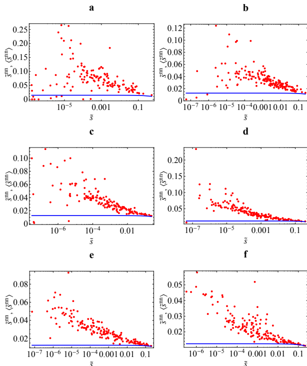
FIG. 6: (Color online) Average nearest neighbor strength \bar{s}_i^{nn} versus strength \bar{s}_i in the 2002 snapshots of the commodity-specific (disaggregated) versions of the real weighted undirected ITN (red points), and corresponding average over the maximum-entropy ensemble with specified strengths (blue solid curves). a) commodity 93; b) commodity 09; c) commodity 39; d) commodity 90; e) commodity 84; f) aggregation of the top 14 commodities (see Ref. [1] for details). From a) to f), the intensity of trade and level of aggregation increases.
