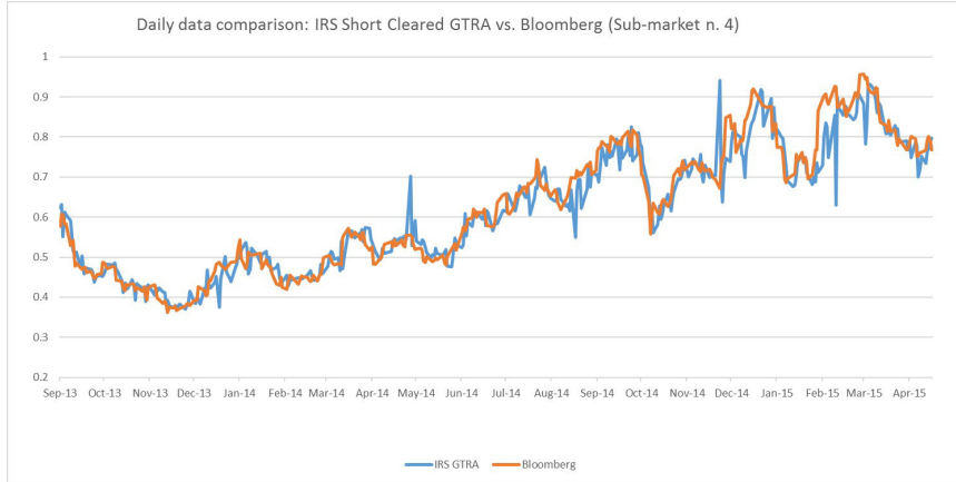
Figure 1: Comparison between GTRA and Bloomberg data
