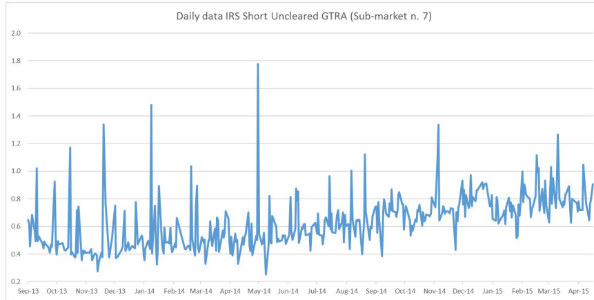
Figure 2: GTRA Price time series for sub-market n. 7
