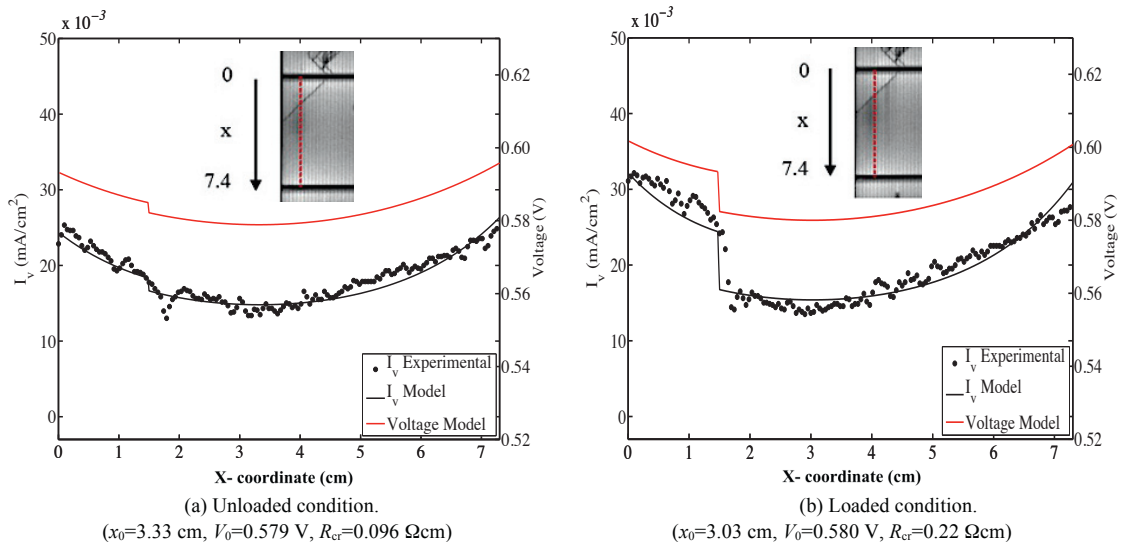
Fig. 3. Vertical current and voltage in a monocrystalline Si cell along a finger crossed by one crack: (a) unloaded and (b) loaded conditions.
