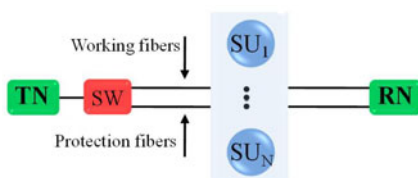
Fig. 2 Shared protection.
