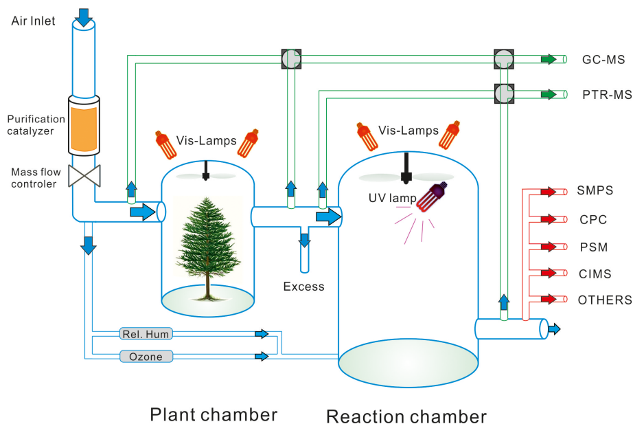
Figure 1. A schematic illustration of the Juelich Plant Chamber (JPAC) setup as it was during the experiments presented here.
