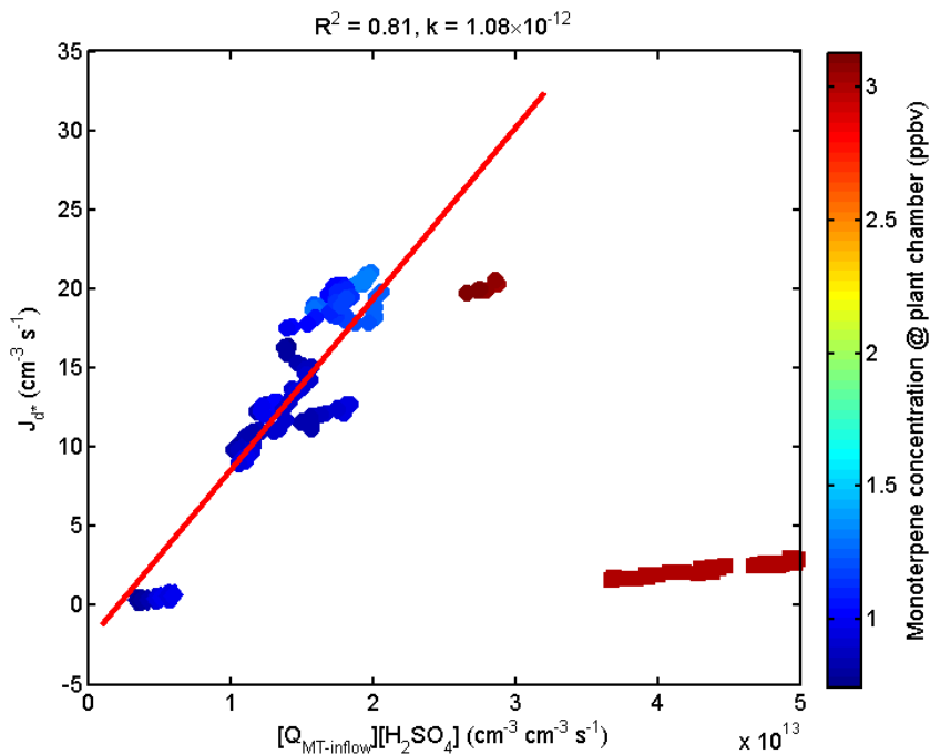
Figure 5. Particle formation rates ( J ) as function of the product of BVOC inflow and sulphuric acid concentration. Marker colours indicate the corresponding monoterpene concentration from the inlet flow of JPAC reaction chamber.
