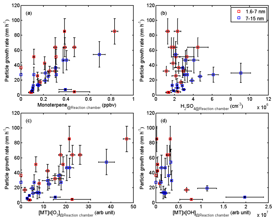
Figure 6. Particle growth rates (GR) at the beginning of the particle formation burst as function of (a) monoterpene concentrations in the JPAC reaction chamber, (b) H 2 SO 4 concentrations in the JPAC reaction chamber. (c) Proxy concentrations of oxidation products of monoterpenes by O 3 in the JPAC reaction chamber (d) proxy concentrations of oxidation products of monoterpenes by OH in the JPAC reaction chamber. Red squares are growth rates of particles ranging from 1.6–7 nm, and blue markers indicates growth rates of particles with diameter of 7–15 nm.
