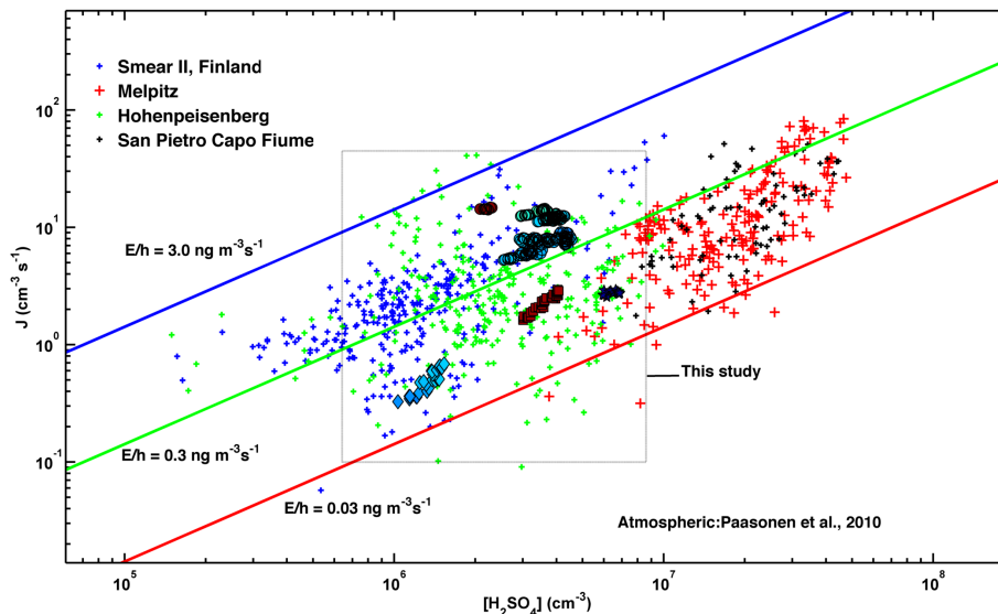
Figure 8. Comparison of our results to atmospheric formation rate studies as reported in Paasonen et al. (2010). Nucleation parameterizations of the form J = K_E \cdot E/h \cdot [H_2SO_4] , with K_E = 4.5 \times 10^{-6} \text{ m}^3 \text{ ng}^{-1} and three different source rates E/h are shown together with measured data points.
