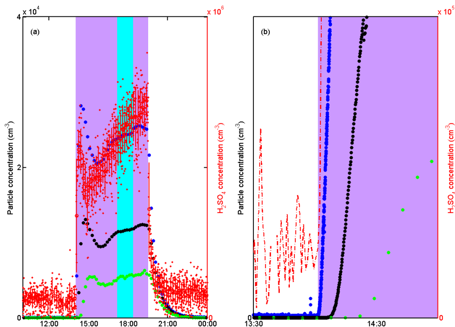
Figure 3. (a) A time series of PSM (blue markers), CPC (black), and CIMS (red) data at the start of one event. The purple area illustrates the time period that UV light was switched on in the reaction chamber. The area shaded blue is the steady-state period from which the particle formation rate was obtained. Sub-figure (b) shows the zoomed-in time delay of particle formation after turning the UV light on, which was used to verify that particles are measured very close to their formation sizes.
