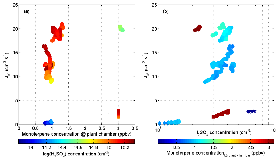
Figure 4. (a) Particle formation rates ( J ) as function of BVOC concentration, and marker colours indicate the corresponding H 2 SO 4 concentrations in log scales. (b) Particle formation rates ( J ) as function of H 2 SO 4 concentrations. Marker colours indicate the corresponding BVOC concentration from the inlet flow. Diamond markers correspond to experiments with no ozone; square markers show data from alpha-pinene experiments; star markers show a zero experiment with no BVOC added.
