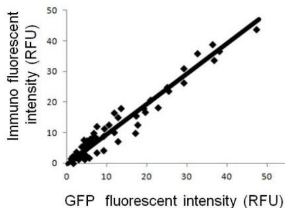
Figure 1. Relationship between fluorescent intensity of GFP and total GluR immunofluorescence.
