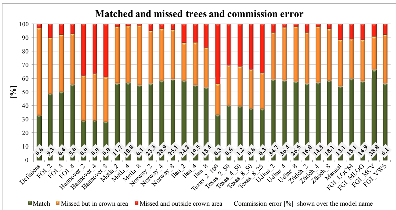
Figure 6. The percentages of matched and missed trees and the commission error (extra trees in the model).
