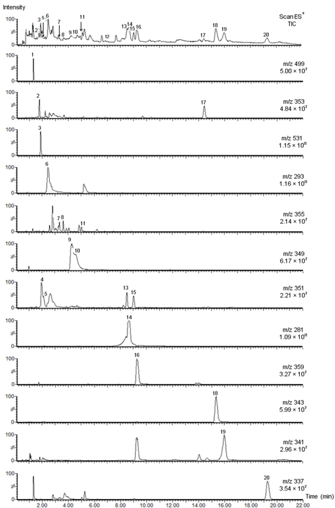
Figure 2. Extracted iongrams (ESI + ) of UPLC-PDA-MS-total ion current (TIC) analysis of R. stricta alkaloids. Data for vincadifformine (12) is presented in Figure S3.
