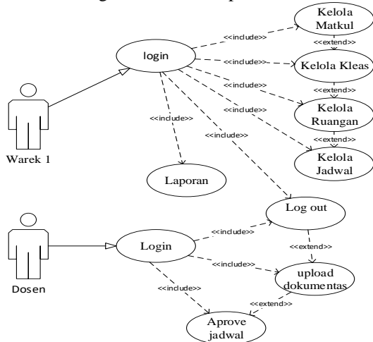
Gambar 4 Usecase Diagram
