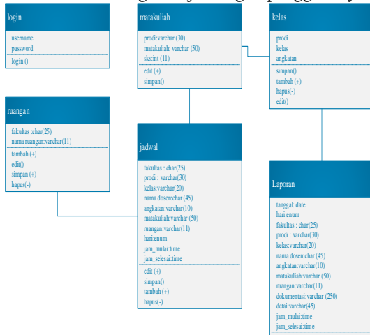
Gambar 7 Class Diagram Sistem E-MONEV
