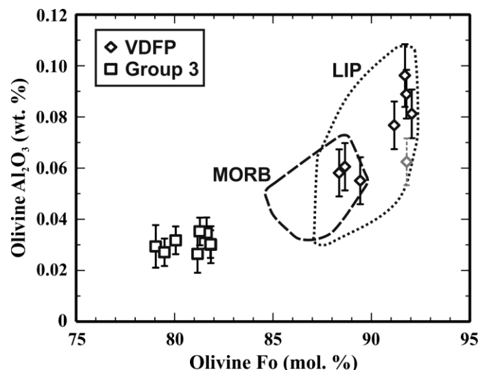
Fig. 3. Olivine Fo vs. olivine \text{Al}_2\text{O}_3 for the Vestfjella depleted ferropicrite suite (VDFP) and Group 3 dykes. Vestfjella olivine–spinel pair that is suspected to be out of equilibrium is shown with a grey symbol and stippled error bars (see Section 5.2.). LIP and MORB fields are after Coogan et al. (2014). The re-equilibrated olivines of the MORBs from the Siqueiros transform fault are not included (Coogan et al., 2014). Error bars ( 1\sigma ) either represent the analytical error or natural variation in olivine \text{Al}_2\text{O}_3 , whichever is larger (see Table 1).
