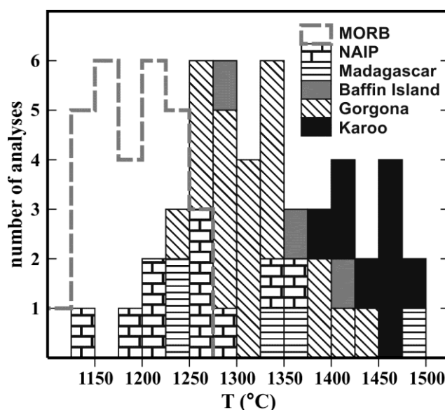
Fig. 6. Histogram that shows Al-in-olivine crystallisation temperatures for MORB and LIP olivine–spinel pairs for which olivine Fo contents are \geq 85 mol%. Data for MORBs and LIPs other than Karoo (this study) are from Coogan et al. (2014).
