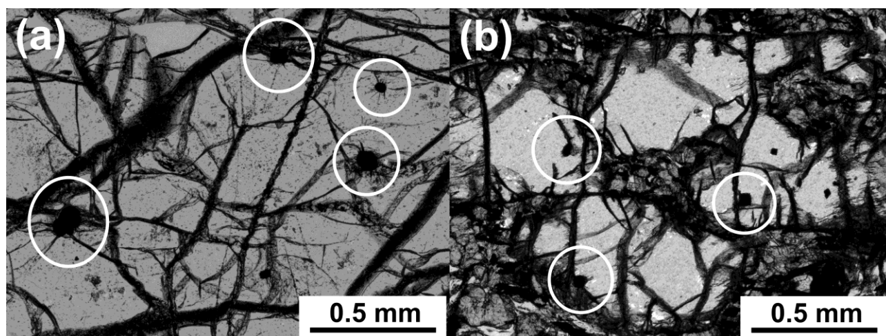
Fig. 2. Spinel inclusions in olivine phenocrysts in plane-polarised light in samples AL/B1b-03 (a: Vestfjella depleted ferropicrite suite) and Z1816.3 (b: Group 3).
