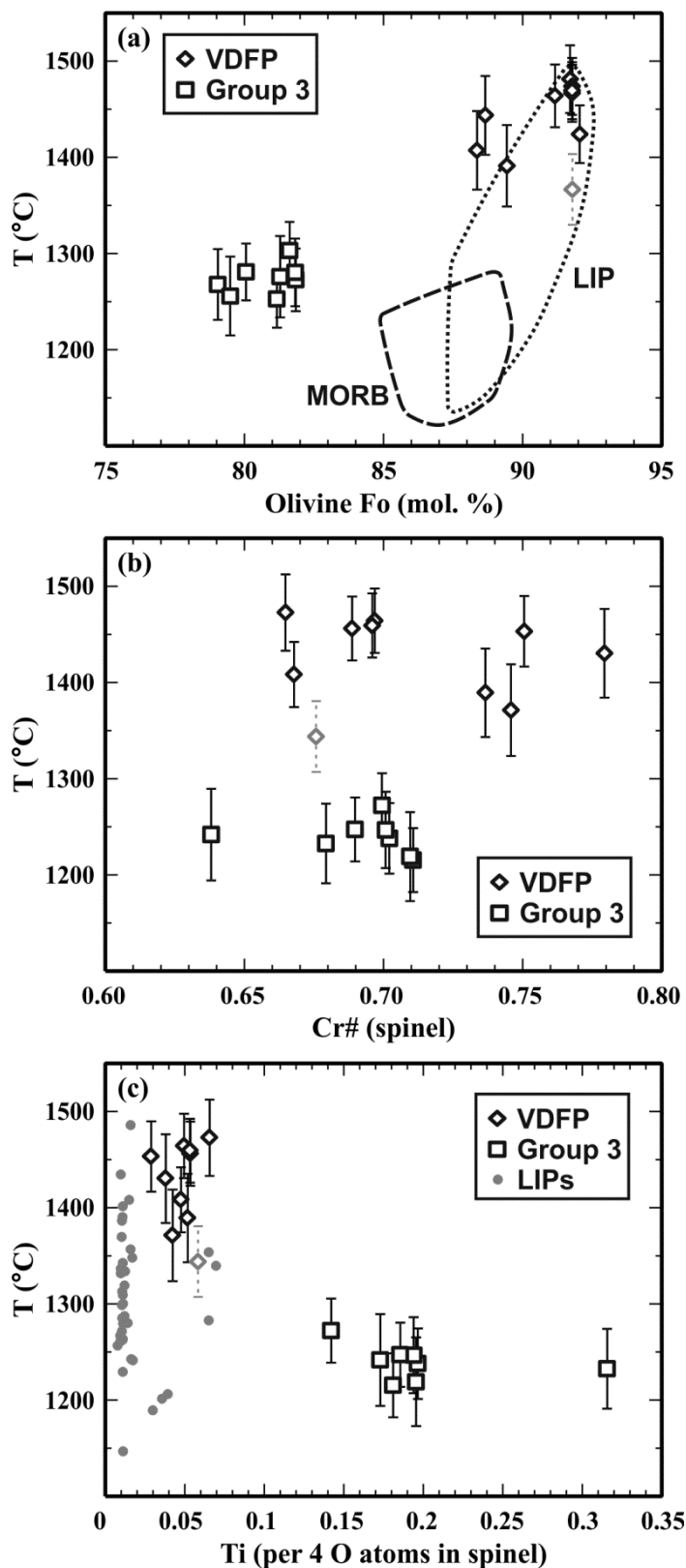
Fig. 5. The results of Al-in-olivine thermometry for the Vestfjella depleted ferropicrite suite and Group 3 dykes shown in olivine Fo vs. T (a), spinel Cr# vs. T (b), and spinel Ti vs. T (c) diagrams. Estimated 1 \sigma errors for the temperatures are shown (see Section 5.2). Vestfjella olivine–spinel pair that is suspected to be out of equilibrium is shown with a grey symbol and stippled error bars (see Section 5.2). LIP and MORB fields in (a) are after Coogan et al. (2014). Olivine–spinel pairs of the MORBs from the Siqueiros transform fault suffer from re-equilibration of the olivines and are not included (Coogan et al., 2014). LIP olivine–spinel pairs with variable Ti^{sp1} analysed by Coogan et al. (2014) shown for reference in (c).
