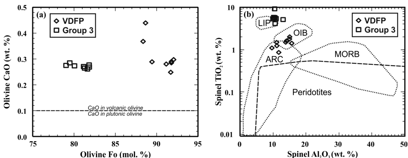
Fig. 4. Mineral chemistry of the analysed samples from the Vestfjella depleted ferropicrite suite (VDFP) and Group 3 dykes shown in olivine Fo vs. olivine CaO (a) and spinel \text{Al}_2\text{O}_3 vs. spinel \text{TiO}_2 diagrams (b). The dashed line that separates volcanic and plutonic olivines on the basis of CaO in (a) is after Simkin and Smith (1970). Spinel discrimination fields in (b) (LIP = large igneous provinces; OIB = oceanic island basalts; MORB = mid-ocean ridge basalts; ARC = island arcs; Peridotites = mantle peridotites) are after Kamenetsky et al. (2001).
