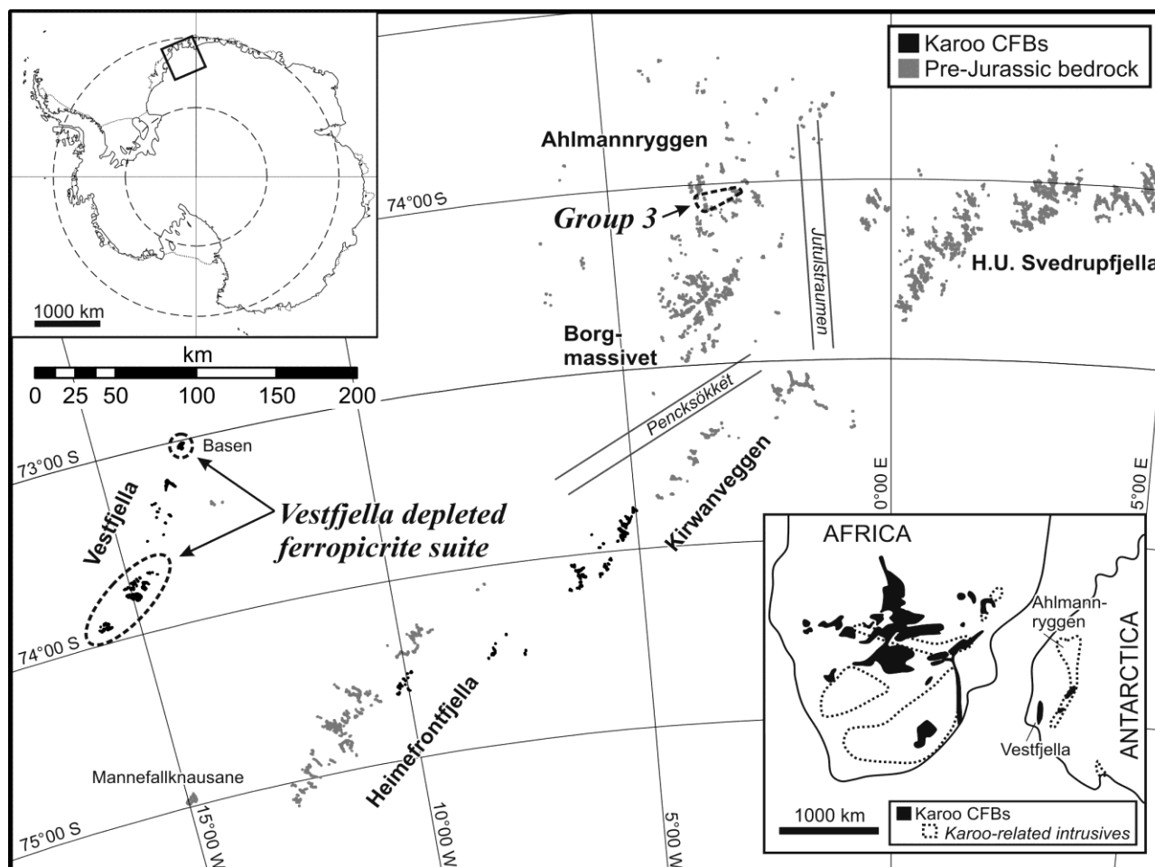
Fig. 1. Outcrop map of western Dronning Maud Land from Vestfjella to H. U. Sverdrupfjella with distribution of Karoo flood basalts and Vestfjella depleted ferropicrite and Ahlmannryggen Group 3 dyke suites. Distribution of Karoo flood basalts and related intrusive rocks in reconstructed Gondwana supercontinent (see Heinonen et al., 2010) is shown in the lower right inset.
