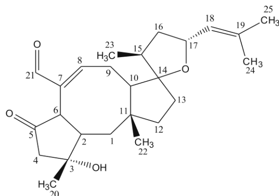
Figure 1. Structure of ophiobolin A.
