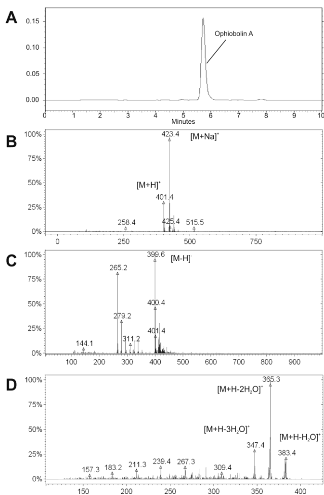
Figure 2. HPLC-UV chromatogram of the purified OPA at 230 nm (A); and the acquired mass spectra by ESI-MS in positive (B) and in negative mode (C); as well as by ESI-MS/MS after the fragmentation of m/z 401.4 in positive mode (D). The characteristic masses were marked.
