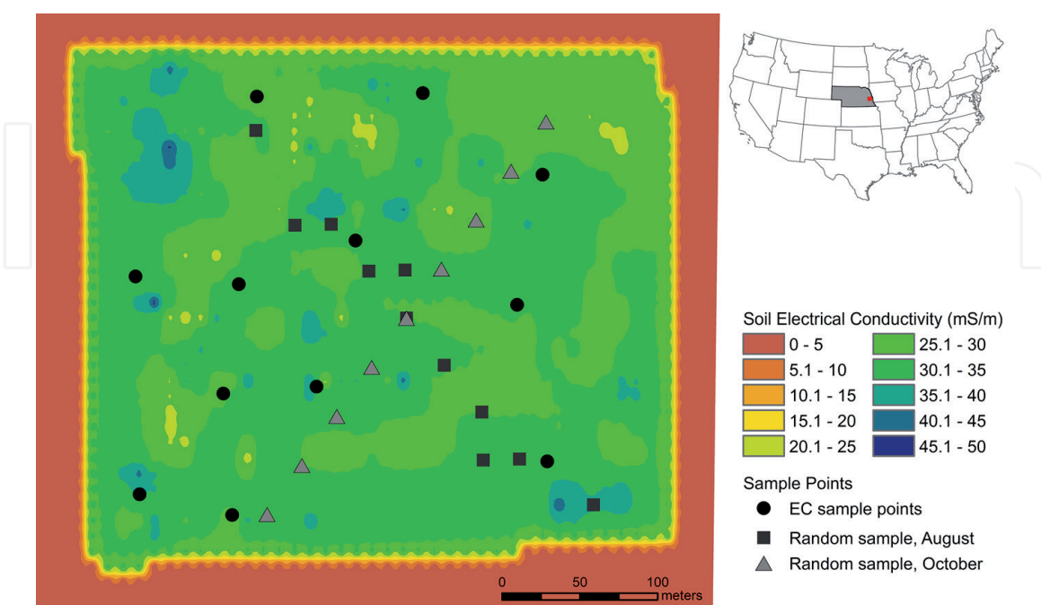
Figure 1. Map showing distribution of soil apparent electrical conductivity (EC a ) mS m^{-1} in brome grass pasture study site. The points on the map indicate locations where soil sample were taken following EC (●) and random August (■) and October (▲)-based techniques. On the right corner is the site location in highlighted state of Nebraska and continental map of USA.
