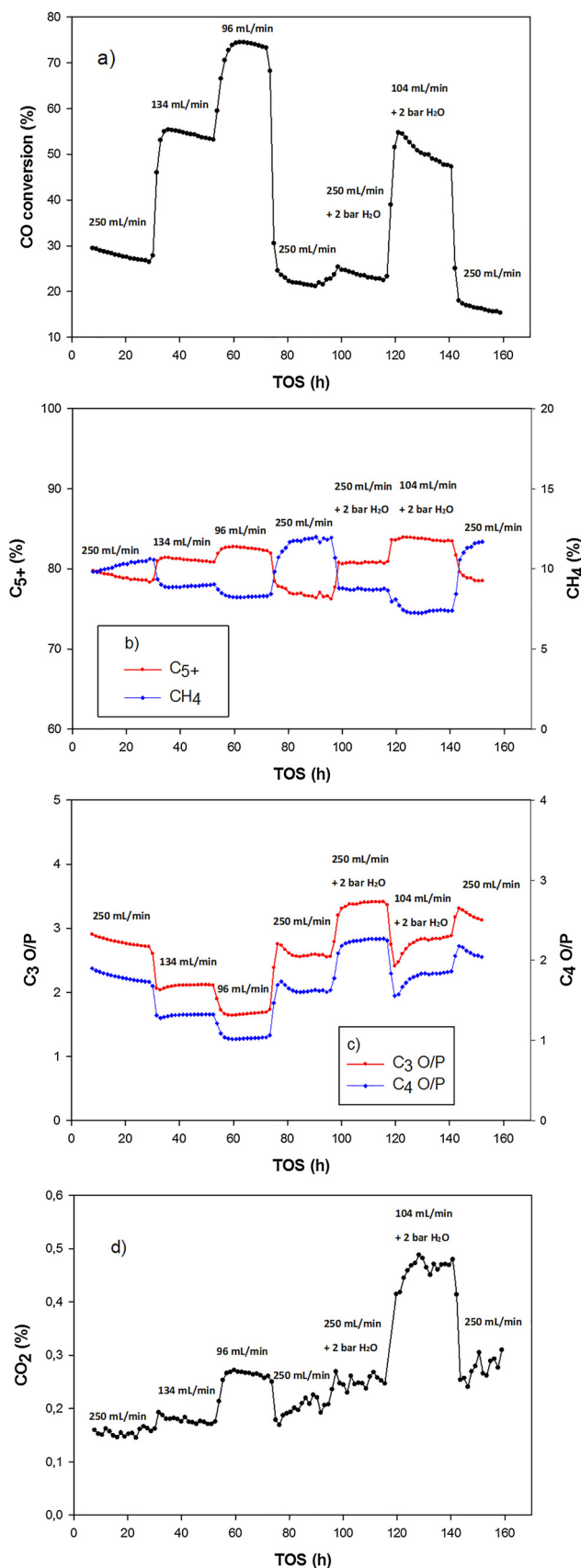
Fig. 1. Catalytic results at different conditions vs Time on Stream (TOS) with H_2/CO = 2.13 at 210\text{ }^\circ\text{C} and 20 bar. a) CO conversion b) Selectivities to C_{5+} and CH_4 c) Olefins to paraffins ratio for C_3 and C_4 hydrocarbons d) Selectivity to CO_2 .
