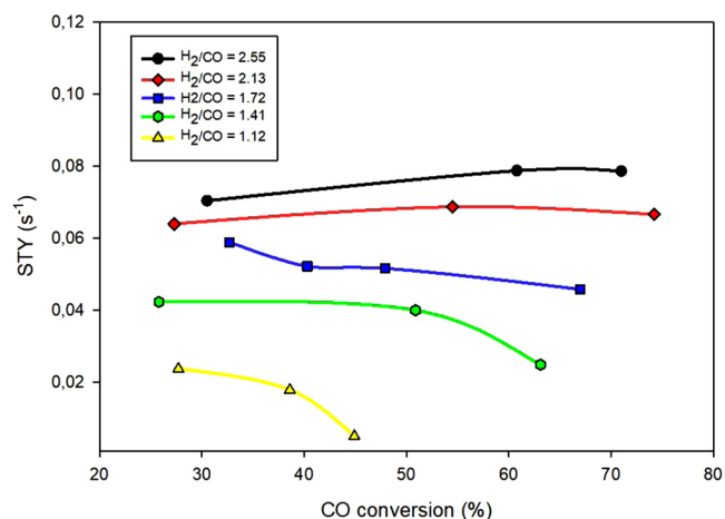
Fig. 2. Catalyst activity reported as site time yields (STY) vs CO conversion with different H_2/CO ratios at 210\text{ }^\circ\text{C} and 20 bar.
