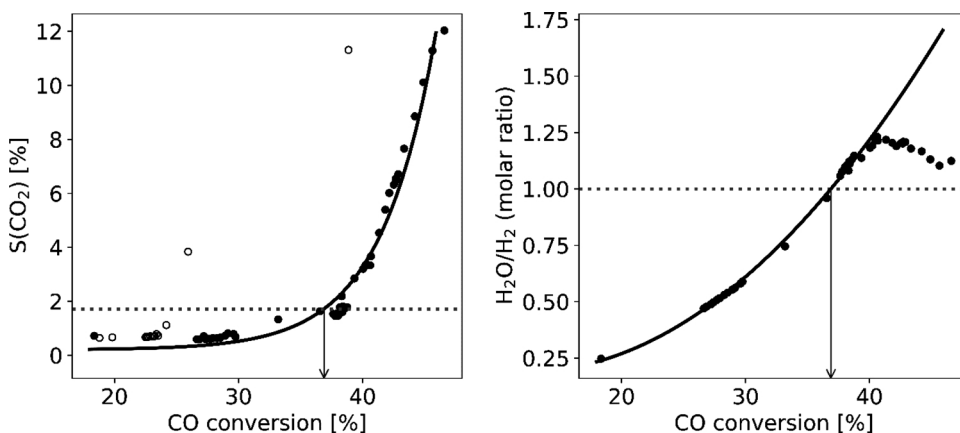
Fig. 3. Relationships between the CO_2 selectivity and CO conversion (left panel), and molar ratio of H_2O and H_2 (right panel) when adding water to the feed. Filled symbols represent data points collected when increasing the conversion, while open symbols denote the return to low conversions. Conditions: H_2/CO = 1.12 , m_{cat} = 4.0\text{ g} , T = 210\text{ }^\circ\text{C} , p = 20\text{ bar} .
