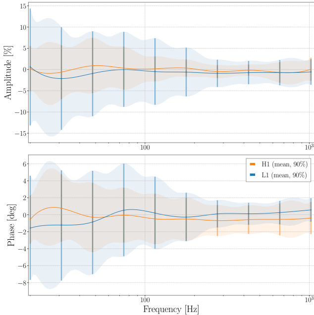
Figure 2. Calibration posteriors for the amplitude (top) and the phase uncertainty (bottom) for both LIGO Hanford (orange) and Livingston (blue) detectors for GW150914. The solid curves shows the mean, while the shaded region represents the 90% confidence intervals. The vertical lines show the locations of the spline points.
