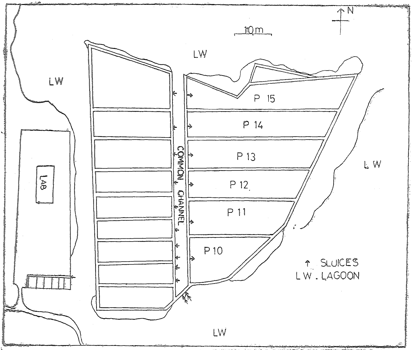
Fig. 1 —The lay out-of the experimental ponds at the Brackishwater Fisheries Station, Pitipana, Negombo.
