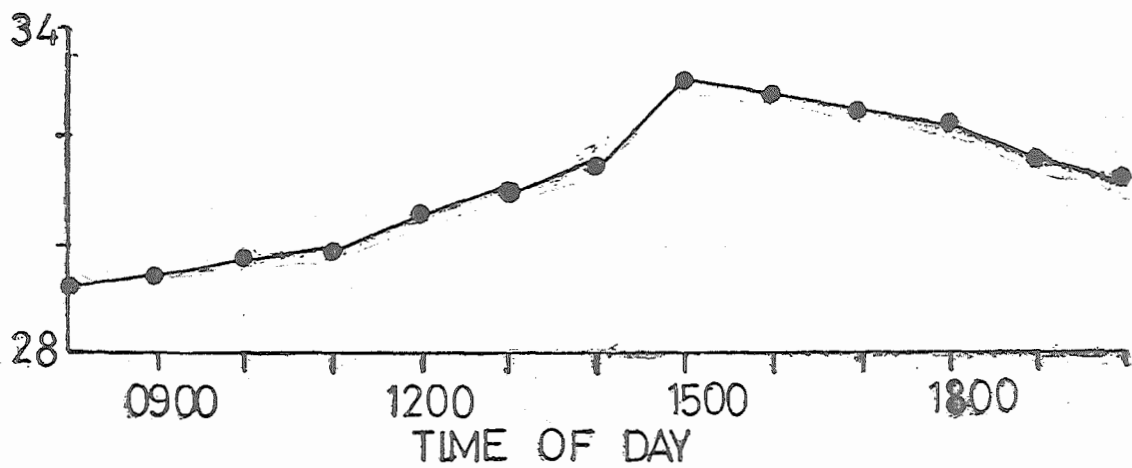
Fig. 2B.—The mean hourly temperature for the Ponds averaged over the months of May and June.
