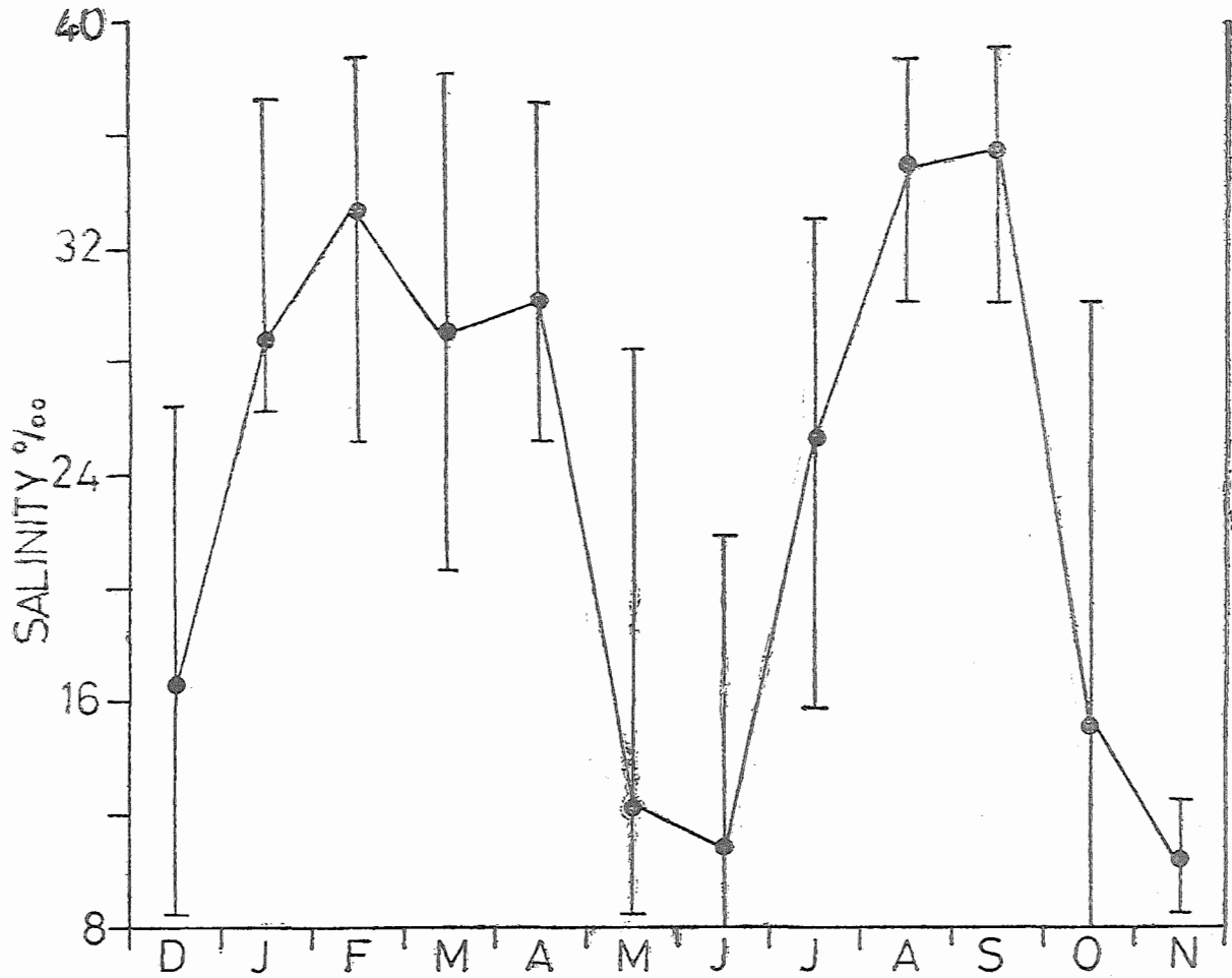
Fig. 3A.—Seasonal variation of the mean monthly salinity of the Ponds (the vertical lines indicate the range in salinity)
