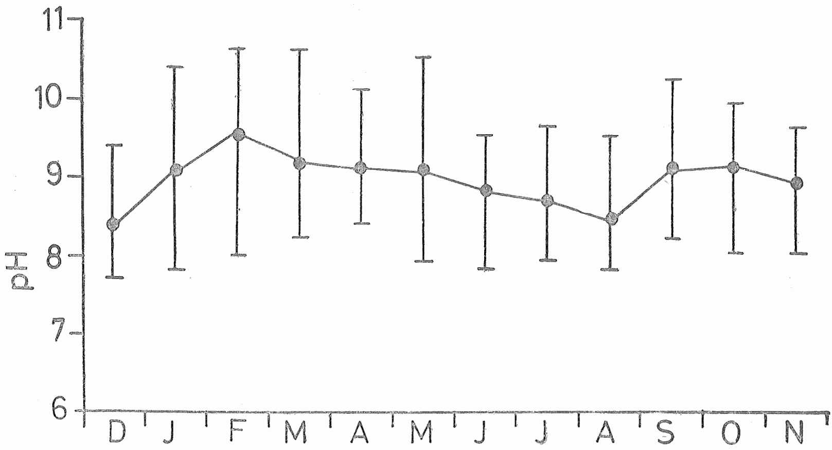
Fig. 4.—Seasonal variation of the mean monthly pH of the Ponds (the vertical lines indicate the range in pH).
