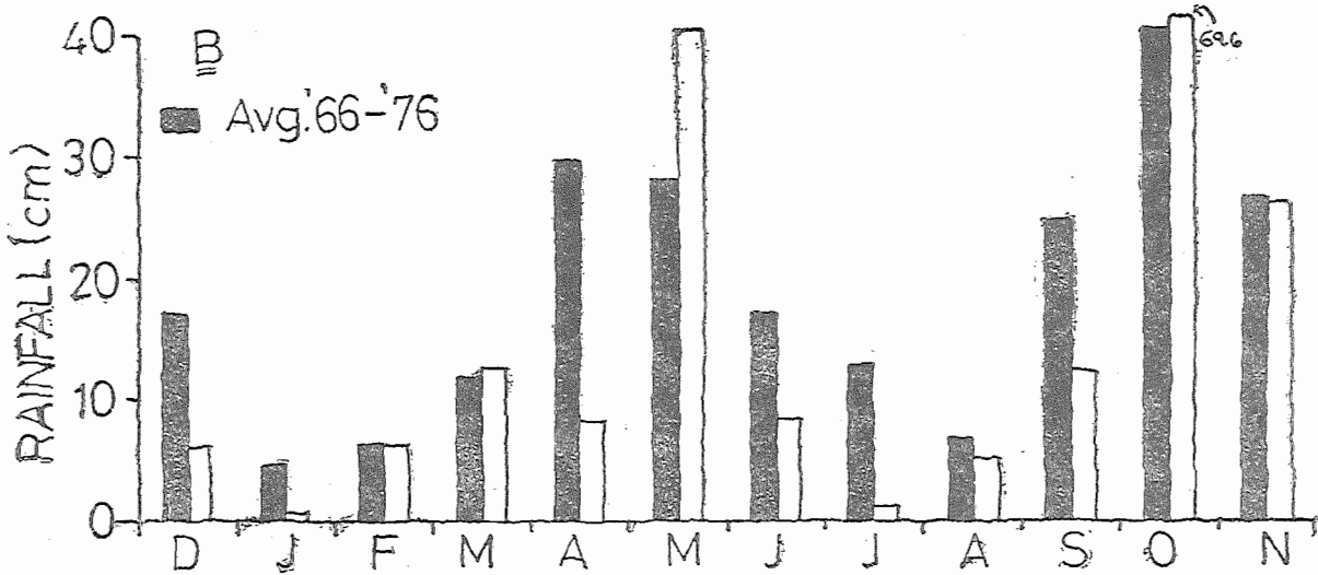
Fig. 3B.—The mean monthly rainfall for Negombo, averaged for the period 1966 to 1976 and the mean rainfall for the experimental period.
