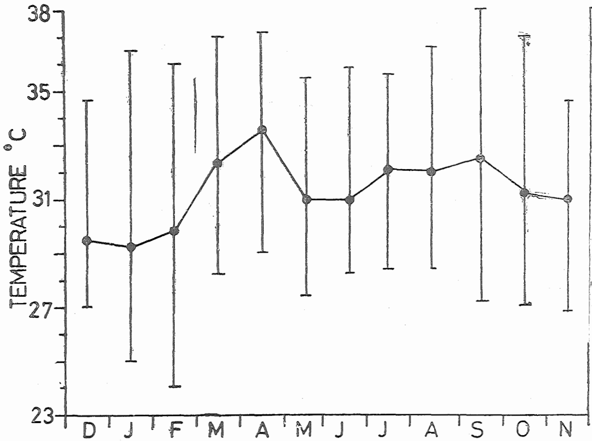
Fig. 2A.—Seasonal variation of the mean monthly temperature of the Ponds (the vertical lines indicate the range for each month).
