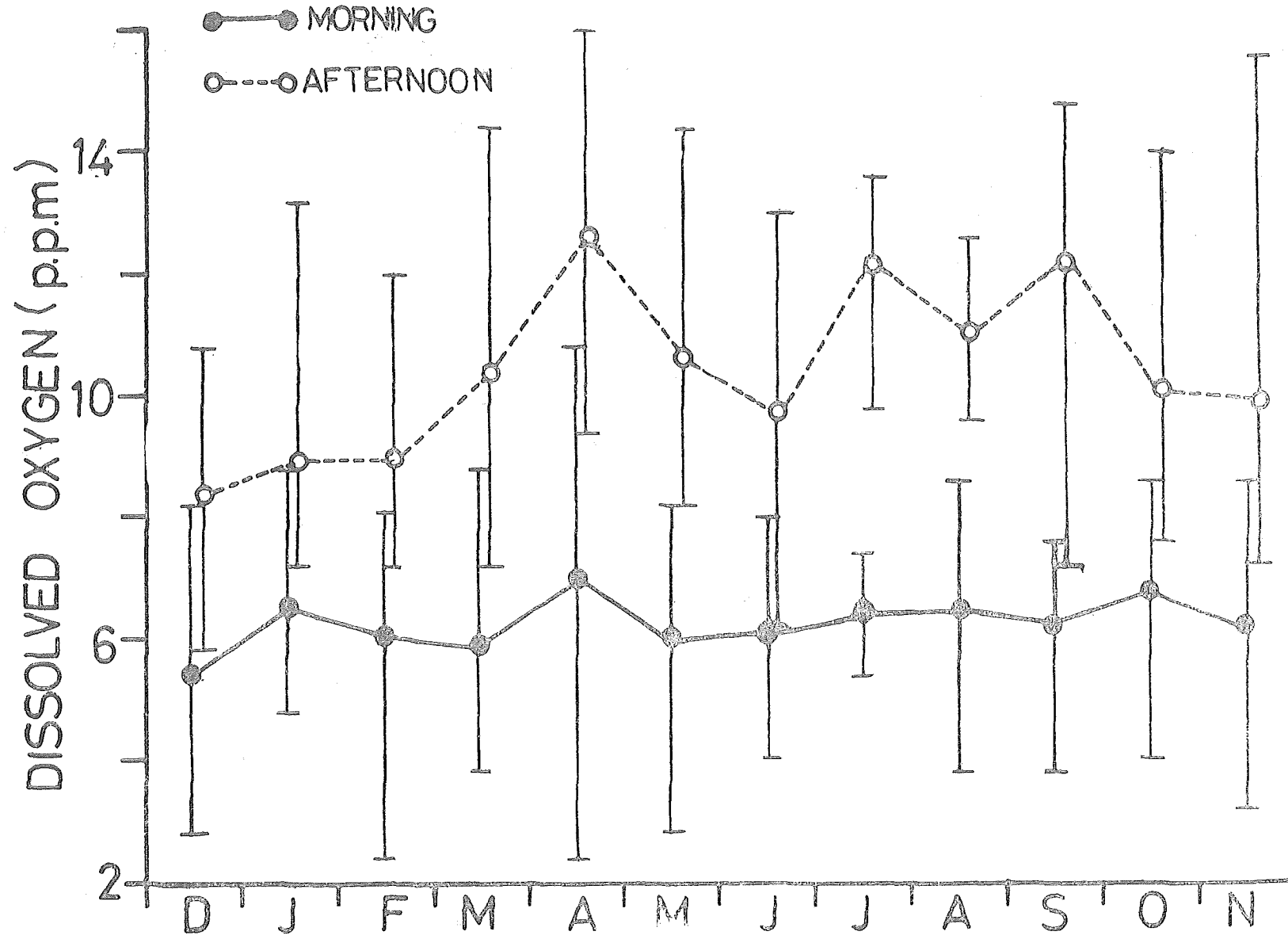
Fig. 5.—The mean monthly dissolved oxygen content of the water in the morning and in the afternoon (the vertical lines indicate the range in d.o. content.)
