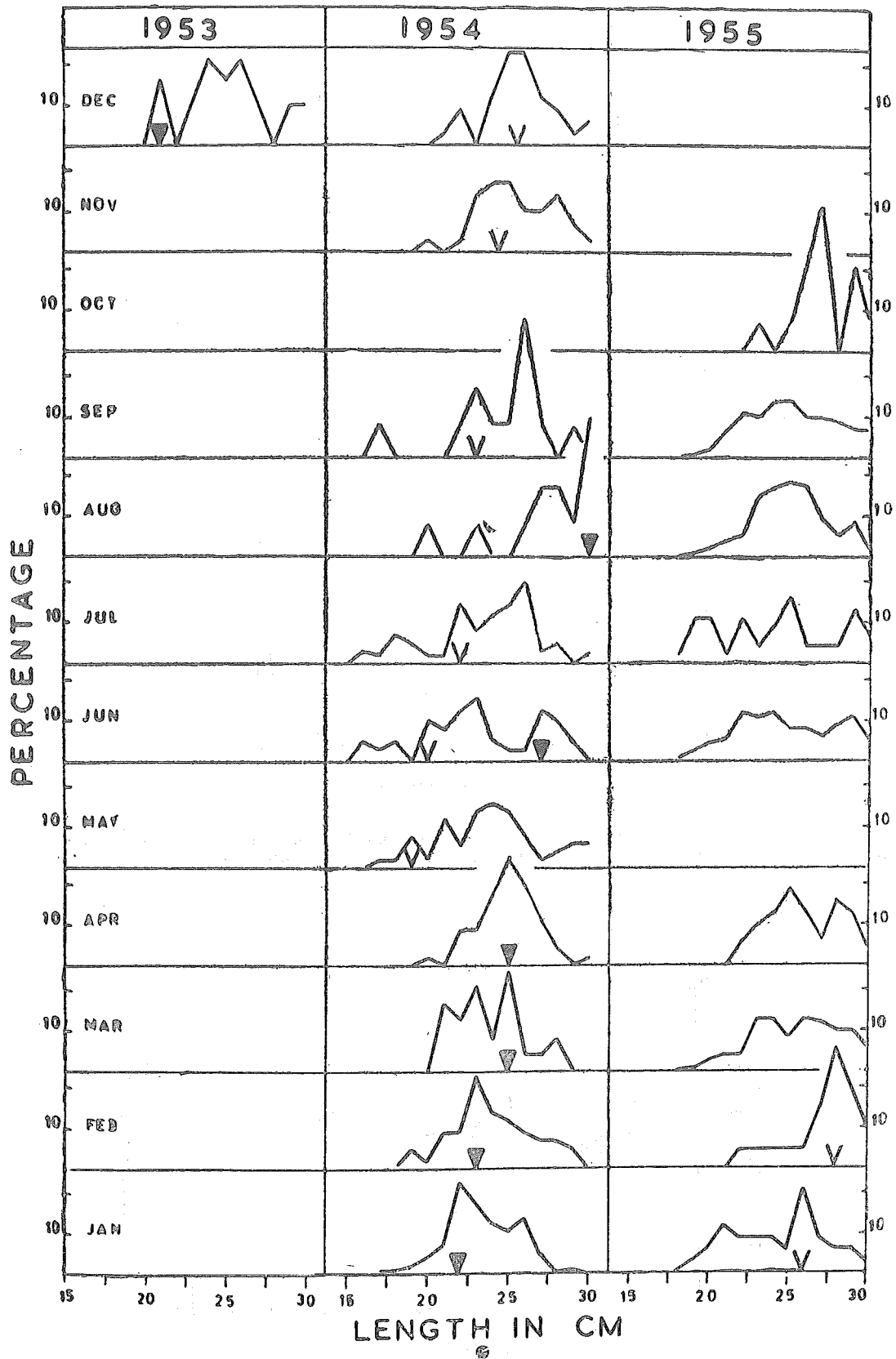
Fig. 3. Monthly length frequency distribution of sea bream ( \leq 30 cm.) for the years 1953-1955. Symbols shown indicate locations of modes used in figure 7.
