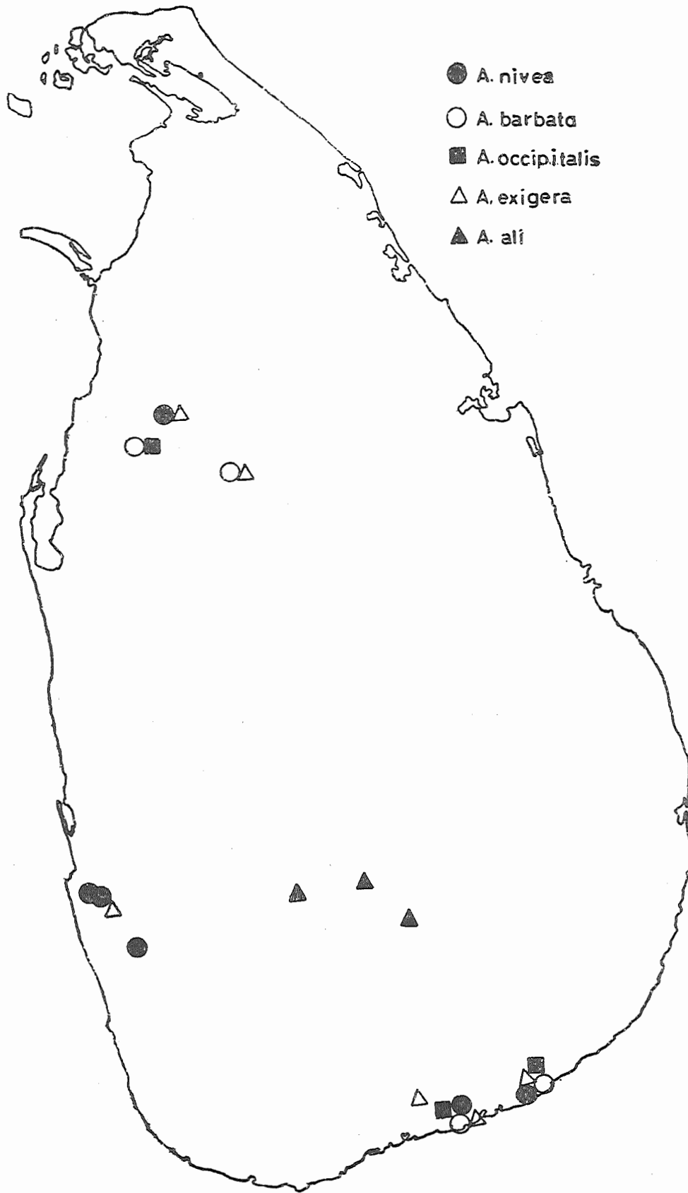
Fig. 4. Distribution of Anisops in Ceylon.
