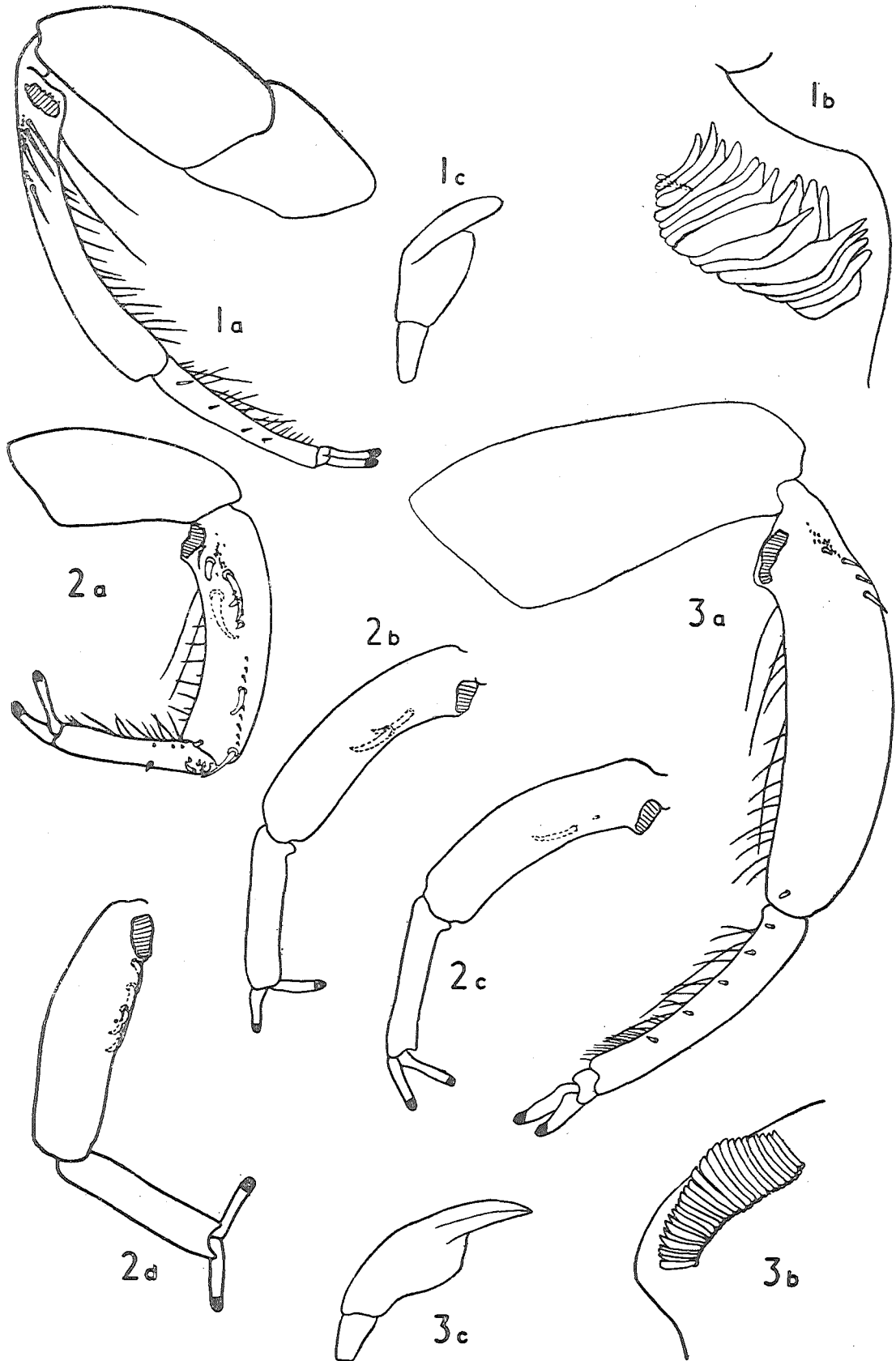
Figs. 1-3: Anisops ali : 1a Chaetotaxy of male foreleg; 1b. Enlarged stridulatory comb; 1c. Rostral prong. Anisops batillifrons : 2a. Male foreleg with one procumbent spine; 2b. Male foreleg with two procumbent spines; 2c. Male foreleg with two procumbent spines; one of which is rudimentary; 2d. Male foreleg with three procumbent spines. Anisops occipitalis : 3a. Chaetotaxy of male foreleg; 3b. Enlarged stridulatory comb; 3c. Rostral prong.
