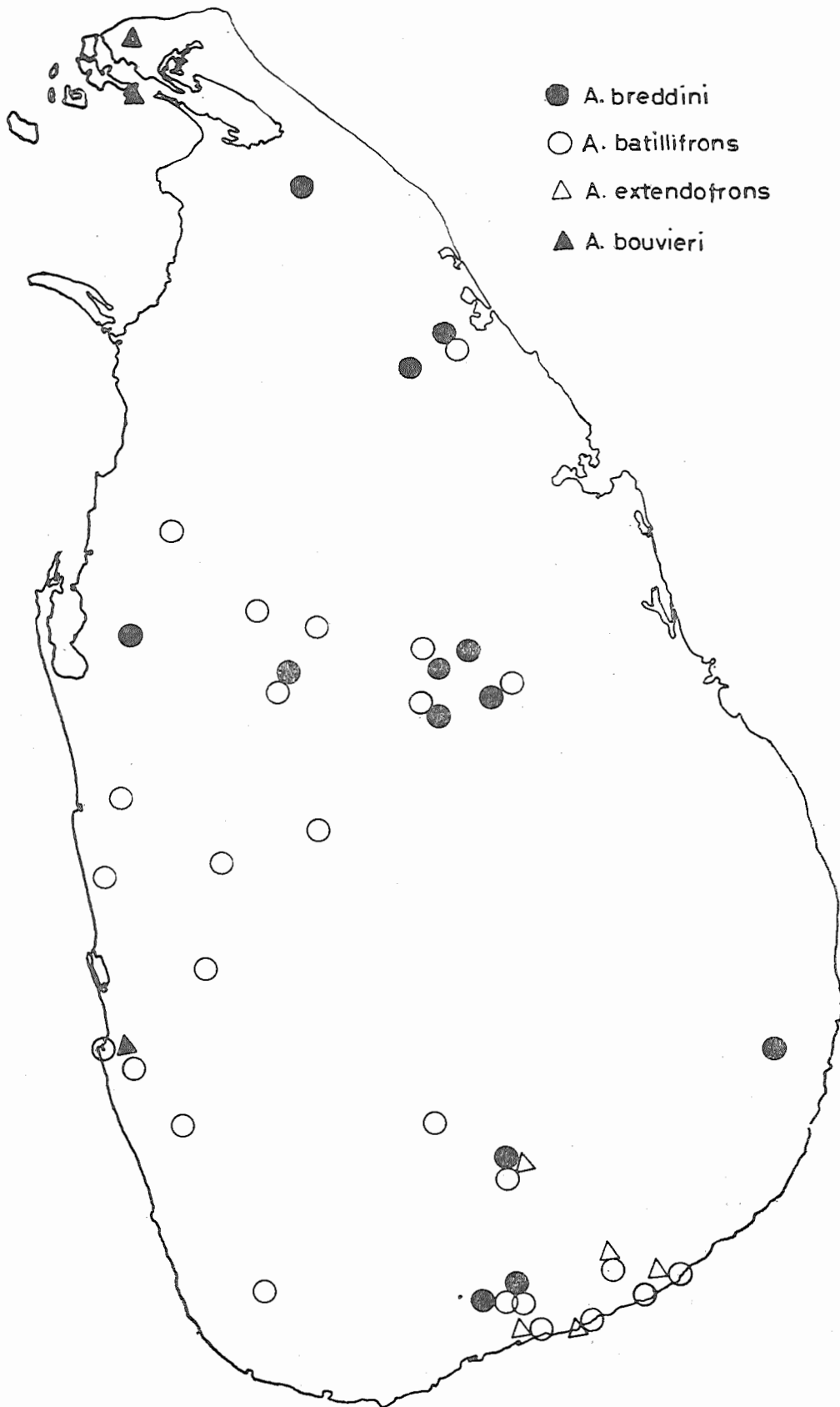
Fig. 5. Distribution of Anisops in Ceylon.
