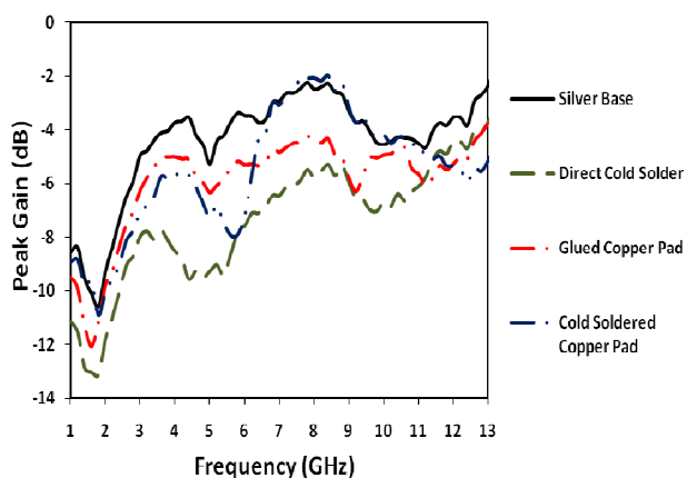
Fig. 6 The measured peak gain of the four antennas.
