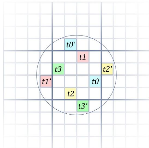
Gambar 6. Sampel RGSS
