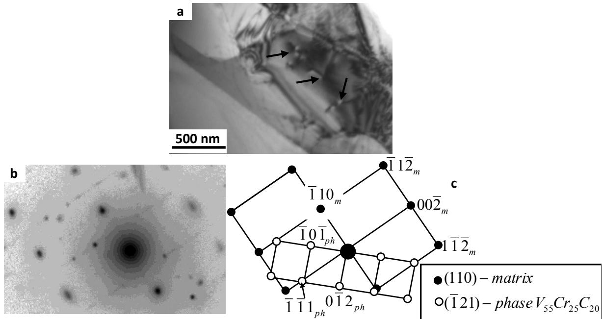
Figure 6. TEM image of the microstructure of the V-4.9Ti-4.8Cr alloy after sintering (a). The arrows point to the particles of carbide V_{55}Cr_{25}C_{20} , fixing dislocations; b - microdiffraction pattern of the section (a); c - its indicated scheme.
