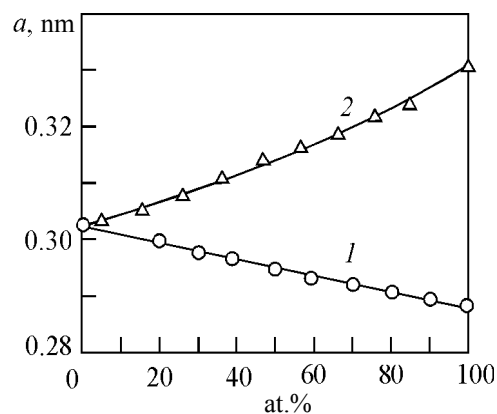
Figure 2. Concentration dependences of crystal lattice parameters of solid solutions V-Cr (curve 1) and V-Ti (curve 2).
