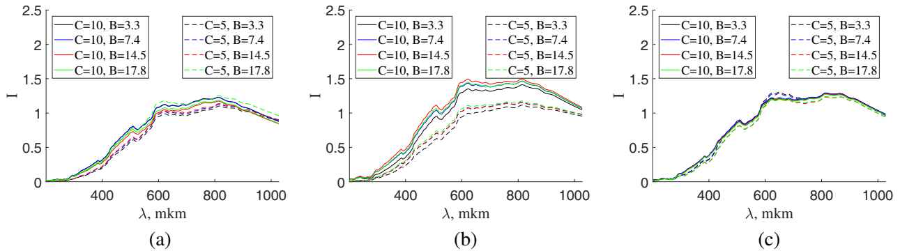
Figure 5. Spectra of THz signal intensity passing through: (a) MF_0, (b) MF_300, (c) MF_500, when Helmholtz coils location No. 3. Here C is the concentration (%), B — magnetic field induction (mT).
