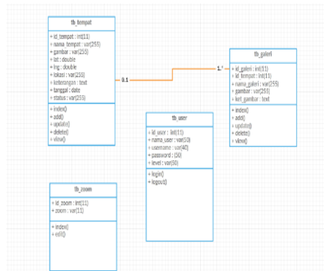
Gambar 10. Class Diagram Damkar
