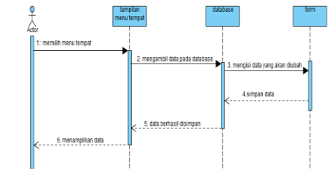
Gambar 8. Sequence Diagram Edit Data Tempat
