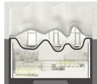
Fig.13: Section
