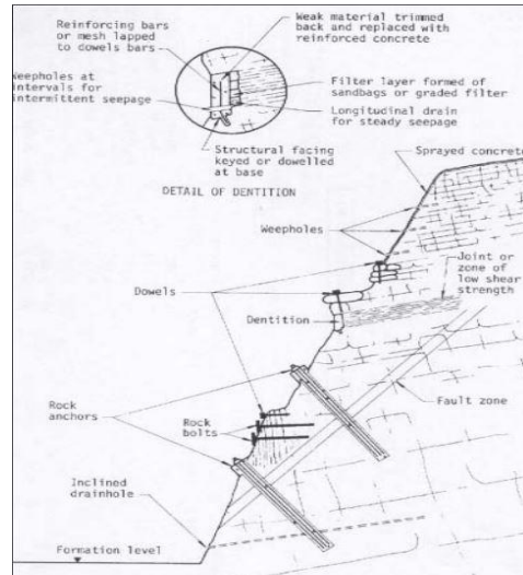
Fig.4: Methods to stabilize a rock slope
