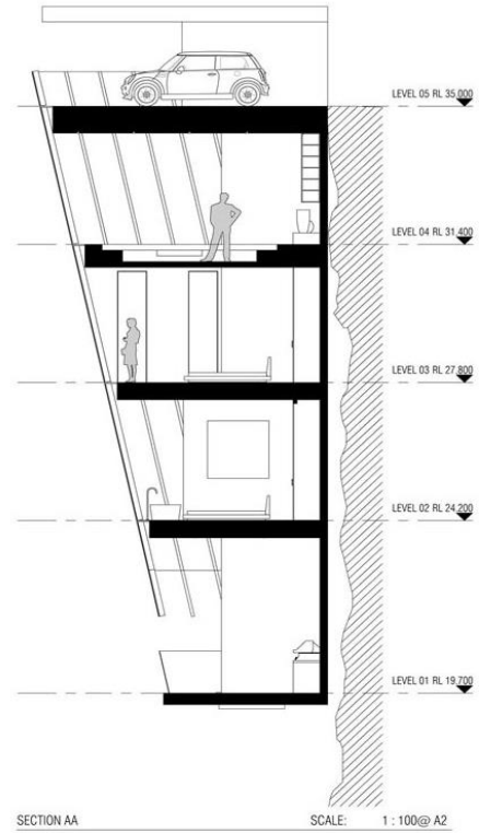
Fig. 10: Section shows the relation of the building with the mountain
