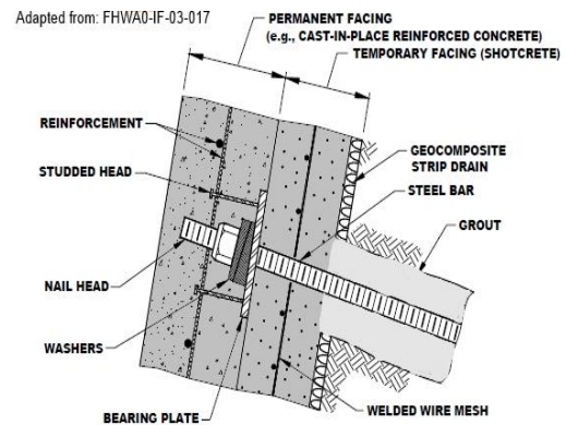
Fig.7: Typical soil nails head plate details
