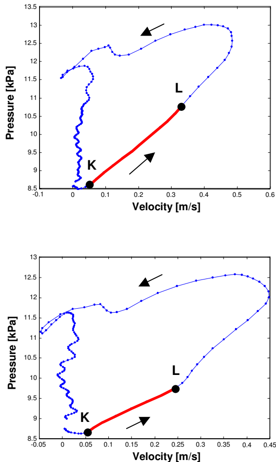
Figure 2. The PU-loop measured in the ascending aorta of dog at control conditions (a), and during abdominal occlusion (b). The initial linear part of the loop is determined using the new algorithm and shown in bold. The arrows indicate the direction of the loop. Sampling points (K) and (L) are the beginning and end of the initial linear part respectively. Although the end of the initial linear part of the PU-loop during control is less obvious than that during occlusion, the new technique accurately detects the length of the linear part in both cases.
