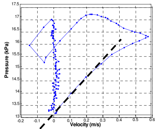
Figure 1. The PU-loop measured in the ascending aorta of dog at control conditions. The initial linear part of the loop, indicating wave speed of 6.6 m/s, is determined by eye and shown in the dashed line.
