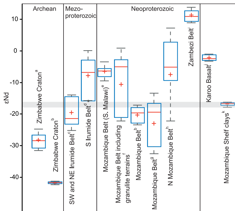
Figure 4. Comparison of \epsilon_{Nd} values obtained from surface clays of the Mozambique Shelf with \epsilon_{Nd} values of whole-rock samples of potential source rocks using box and whisker plots with mean and median indicated by crosses and horizontal red lines, respectively. References: a Jelsma et al., [1996], b Grantham et al., [2011], c De Waele et al., [2006], d Johnson et al., [2007], e Kröner et al., [2001], f Möller et al., [1998], g Vogt et al., [2006], h Hauzenberger et al., [2007], i John et al., [2004], j Jourdan et al., [2007] and k This study.
