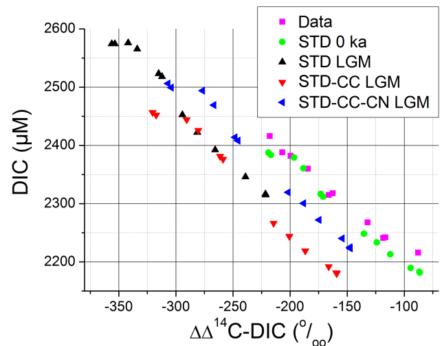
Figure 13. DIC vs. difference between radiocarbon in seawater DIC and atmospheric \text{CO}_2 ( \Delta\Delta^{14}\text{C-DIC} ) at >2000 \text{ m} water depth. Data are mean values for deep water and bottom water boxes derived from water column measurements. Model results are shown for the standard case (STD), for constant circulation (STD-CC), and constant values for circulation and nutrient utilization (STD-CC-CN). LGM refers to model results at 21 ka.
