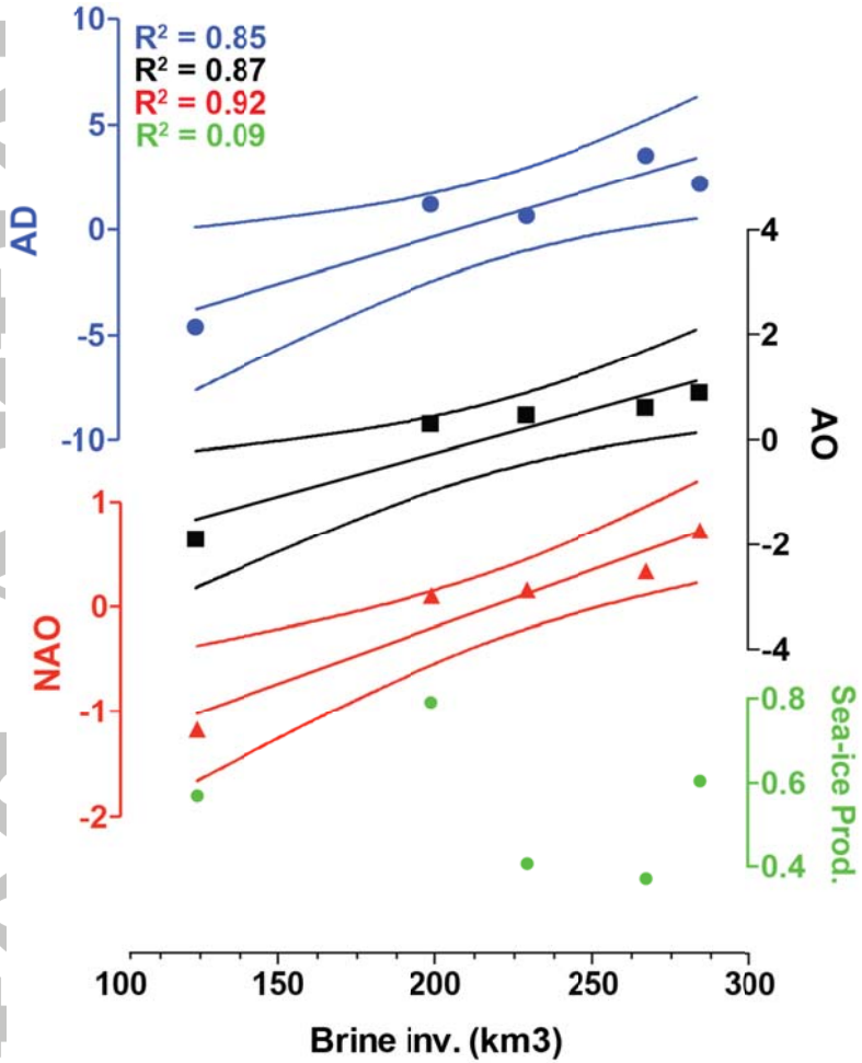
Fig 4. Scatter plot of Winter-Spring Arctic Dipole (AD; DJFMAM; National Oceanic and Atmospheric Administration 2015b) , Arctic Oscillation (AO; JFMA; National Oceanic and Atmospheric Administration 2015) and North Atlantic oscillation (NAO; JFMA; National Oceanic and Atmospheric Administration 2015c) in respect to central Laptev Sea brine inventory. Also, the averaged sea-ice production ( \text{km}^3 \text{ day}^{-1} ) is plotted in green [Preusser et al. , 2014]. Statistical elements (linear fit and 95% confidence envelope) are present only to give the reader a quantitative measure of the relationship and should be considered with cautious because of the small dataset. Note that the R^2 drops to \sim 0.7
