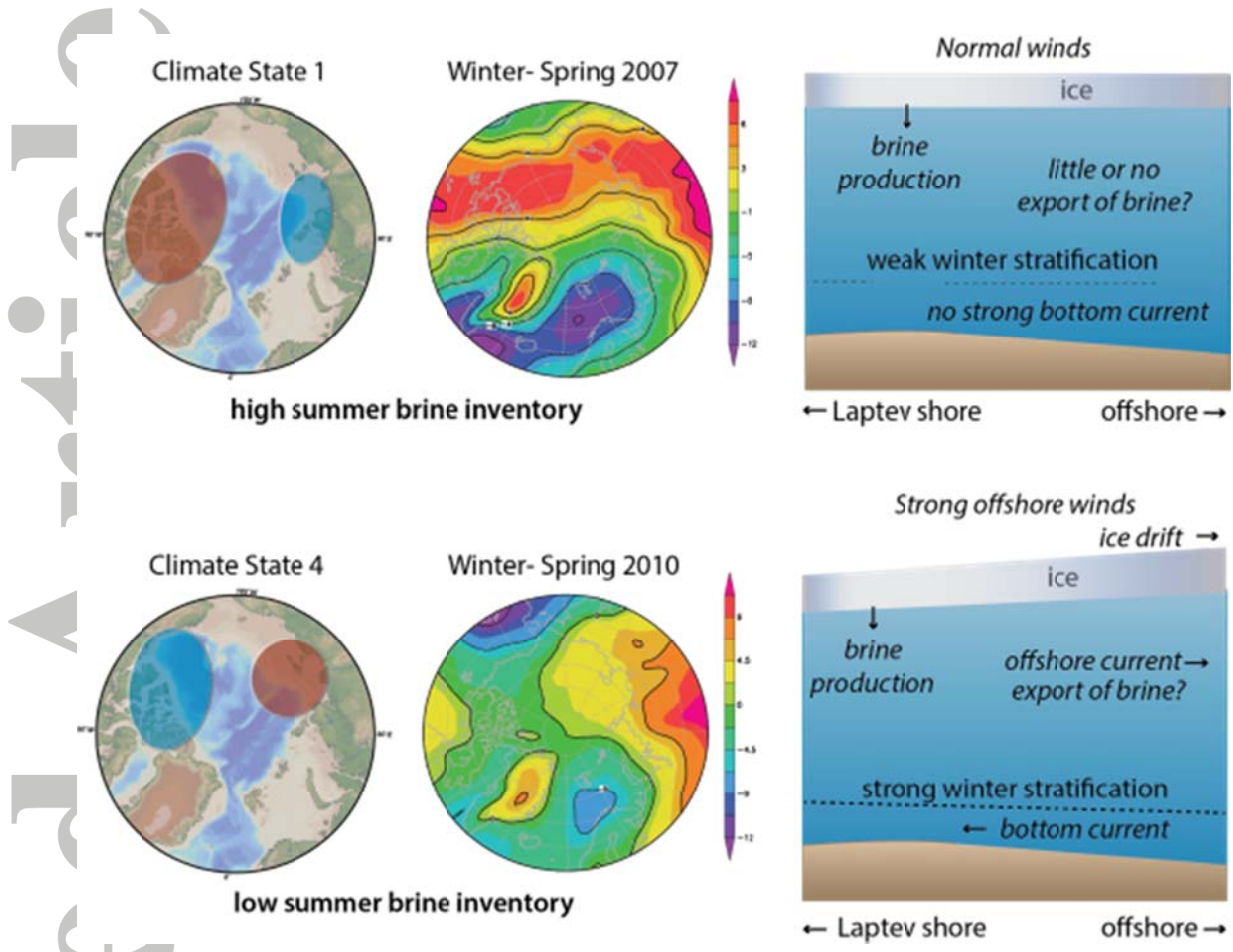
Figure 6. Sketch of the theoretical pressure anomaly for extreme modelled climate state 1 and 4 (respectively double positive and double negative AO and AD) along with the Sea Level pressure anomaly for winter-spring 2007 and 2010 (representative of climate state 1 and 4 in our dataset) and a sketch that illustrates our hypothesis to explain the variability in summer brine inventory between the different climate states.
