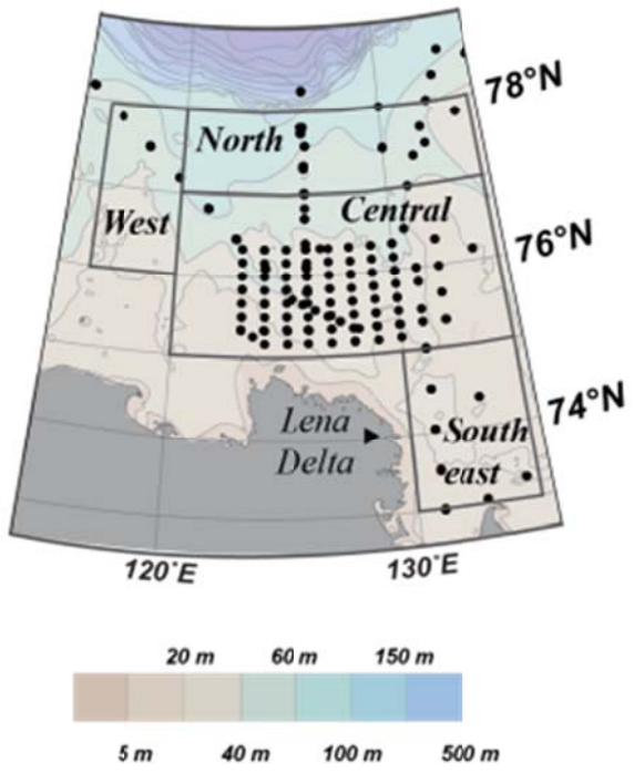
Fig 1. Map of the Laptev Sea shelf with sampling stations location (black dots). Rectangles represent the interpolation zones used to calculate the brine inventory.
