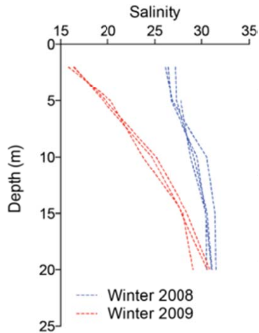
Fig 5. Salinity profiles measured during winters 2008 and 2009 at approximately the same position ( \sim 128.4^{\circ}\text{E} / 74^{\circ}\text{N} ) on the southern limit of the Laptev Sea shelf central zone.
