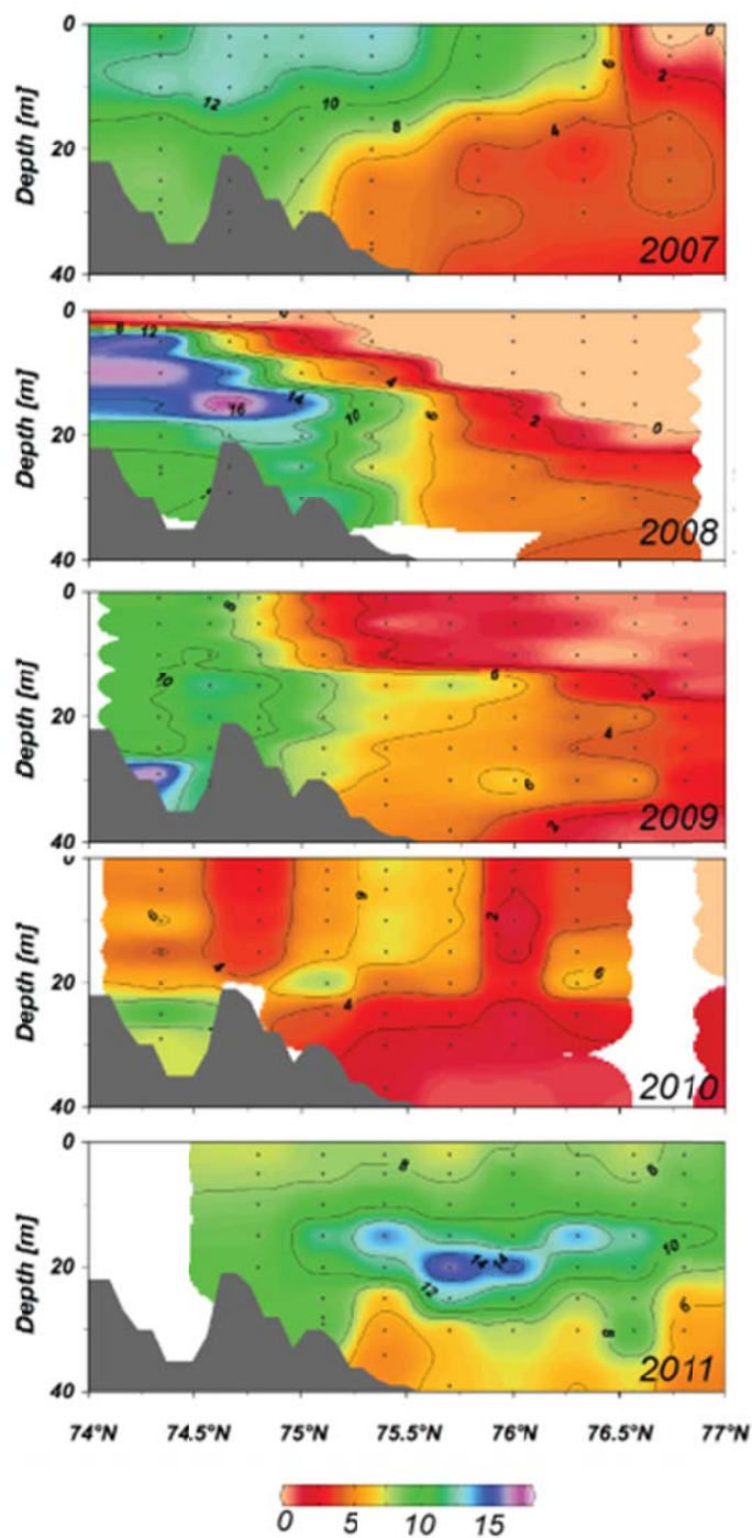
Fig 3. Brine content (in percentage) along 126°E for years 2007-2011. Note that the brine content is the negative fraction of sea-ice meltwater calculated from the water mass analysis (for further explanation see text).
