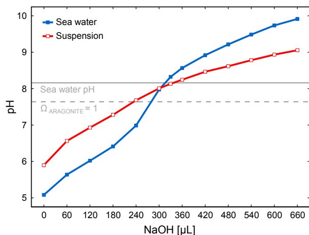
Figure 4. Titration of 500 mL sea water (blue, filled box and line) and 500 mL particle suspension (red, empty box and line) with 3 M NaOH after addition of 150 \mu\text{L} 2.4 M \text{FeCl}_3 solution. The grey solid line indicates the pH of seawater before any manipulation. pH (NBS scale) was measured at 25 ^{\circ}\text{C} with a stationary pH meter (713, METROHM). Calculated aragonite saturation state of \Omega = 1 is represented by the grey dashed line.
