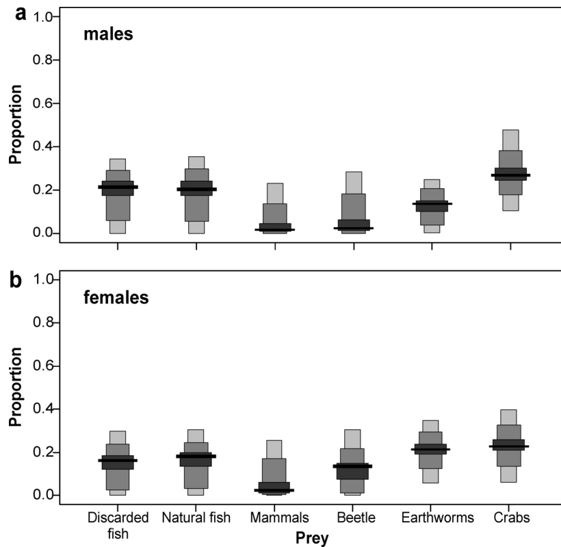
Fig. 11 Proportions of the main food sources, based on \delta^{13}\text{C} and \delta^{15}\text{N} in red blood cells from a male and b female LBBGs breeding on the southern North Sea coast during incubation. Decreasing grey scale and bar width represent 5%, 25%, 75% and 95% probability intervals derived from stable isotope mixing model, Stable Isotope Analysis in R (R package siar 4.2)
