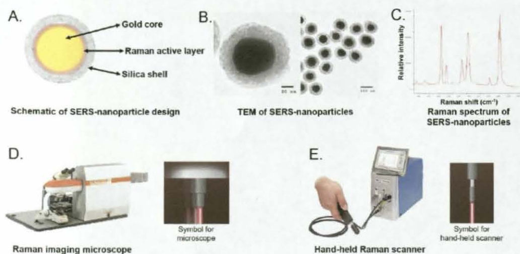
Figure 1. (A) Diagram of the SERS-nanoparticle design, depicting the gold core, Raman reporter layer (4,4'-dipyridyl), and dye-encapsulating silica shell. (B) Transmission electron microscopy images of the SERS nanoparticles. (C) Unique Raman "fingerprint" spectrum of the SERS nanoparticles (acquisition time = 1s, 100 mW laser power). (D) Raman microscope used to acquire images in this study (adjacent schematic serves as the symbol for the microscope in the remaining figures). (E) Hand-held Raman scanner (adjacent schematic serves as the symbol for the microscope in the remaining figures).
