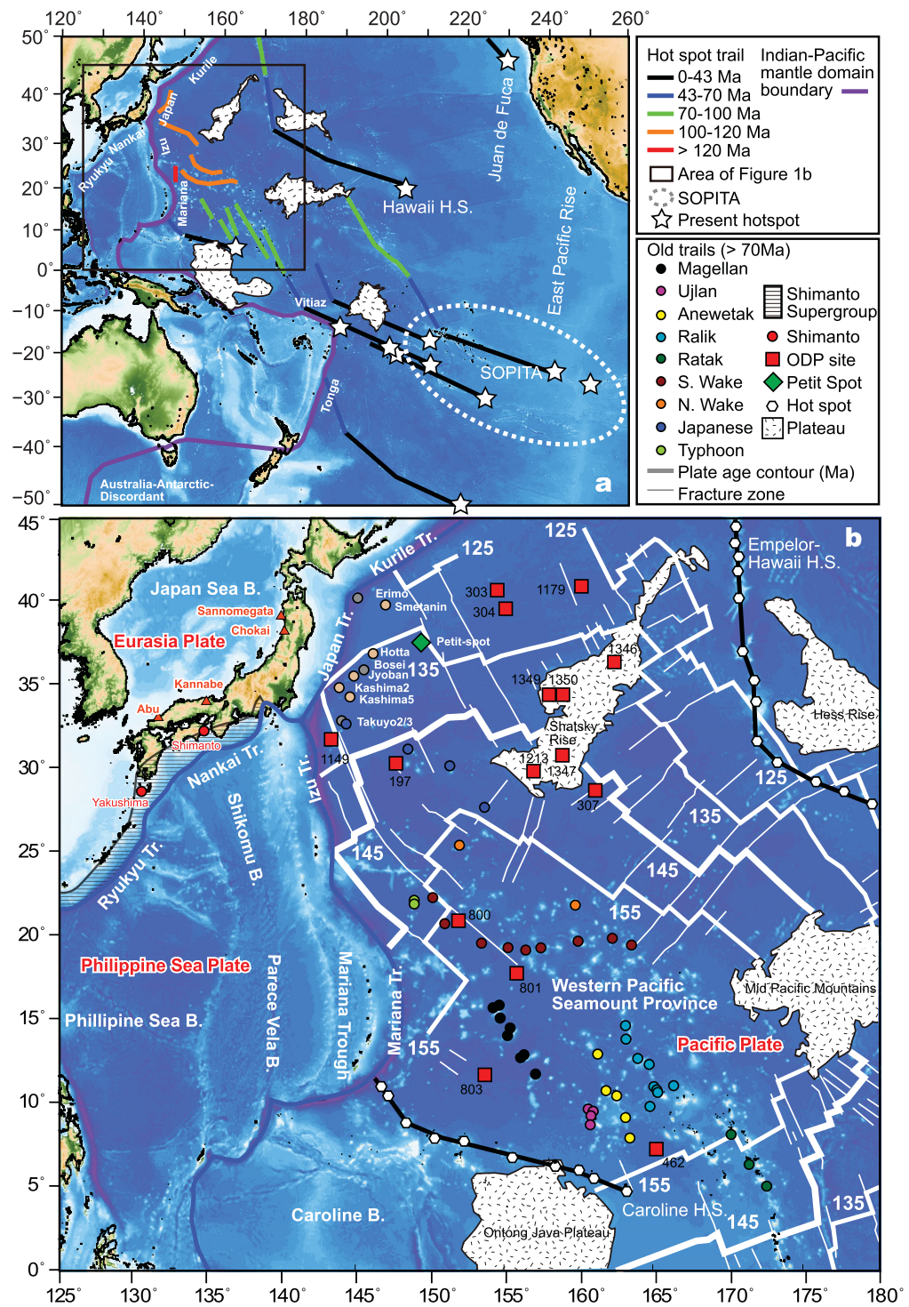
Figure 1. Map showing the Indian-Pacific mantle domain boundary, hotspot tracks, ridges, and subduction zones in the (a) Pacific and (b) western Pacific. Hotspot tracks, rises, and plateaus in Figure 1a are from Condie [2001]. Locations of the MORB and OIB samples used in this study are shown in Figure 1b. Borehole location data were obtained from the IODP web site at http://www.iodp.org/borehole-map . Thick white lines with numbers show ages of the Pacific plate, and thin lines show transform faults [ Nakanishi et al. , 1989]. The SOPITA hotspot trails in Figures 1a and 1b are from Koppers et al. [2003]. Tr: trench; B: basin; HS: hotspot.
