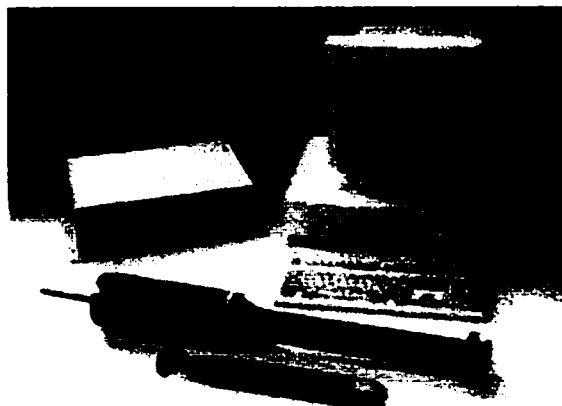
Figure 2.10: Photo from Sippican brochure, showing XCP probe and surface float/transmitter along with computer and MK-10 signal processor/receiver. More info available at http://www.sippican.com/expendable.probes.html
