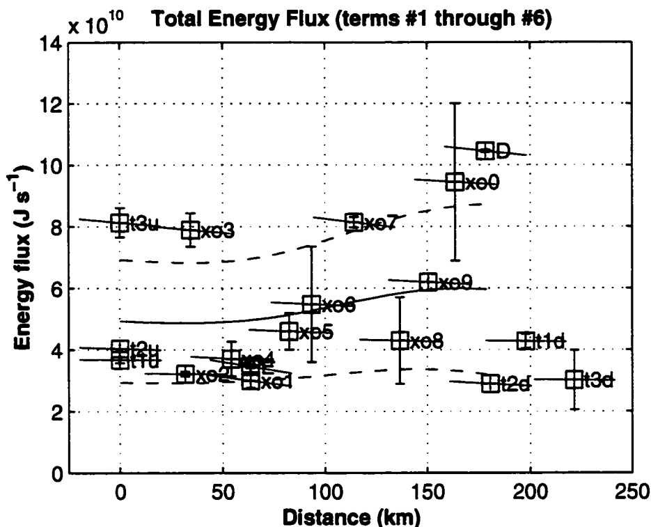
Figure 6.13: Total energy flux ( \iint_A (\mathbf{F}^{\text{tot}} \cdot \hat{\mathbf{j}}) dz dx ) observed at each of 18 sections across the overflow. Values plotted are the sum of all six panels in Fig. 6.12. Slanted lines at each section indicate the rate of decrease expected from bottom stress measurements (Eq. 6.26). The solid curve is a smoothing of the energy flux values using a 75 km Gaussian window, with the dashed curves indicating the envelope of 1\sigma variance (weighted with the same filter).
