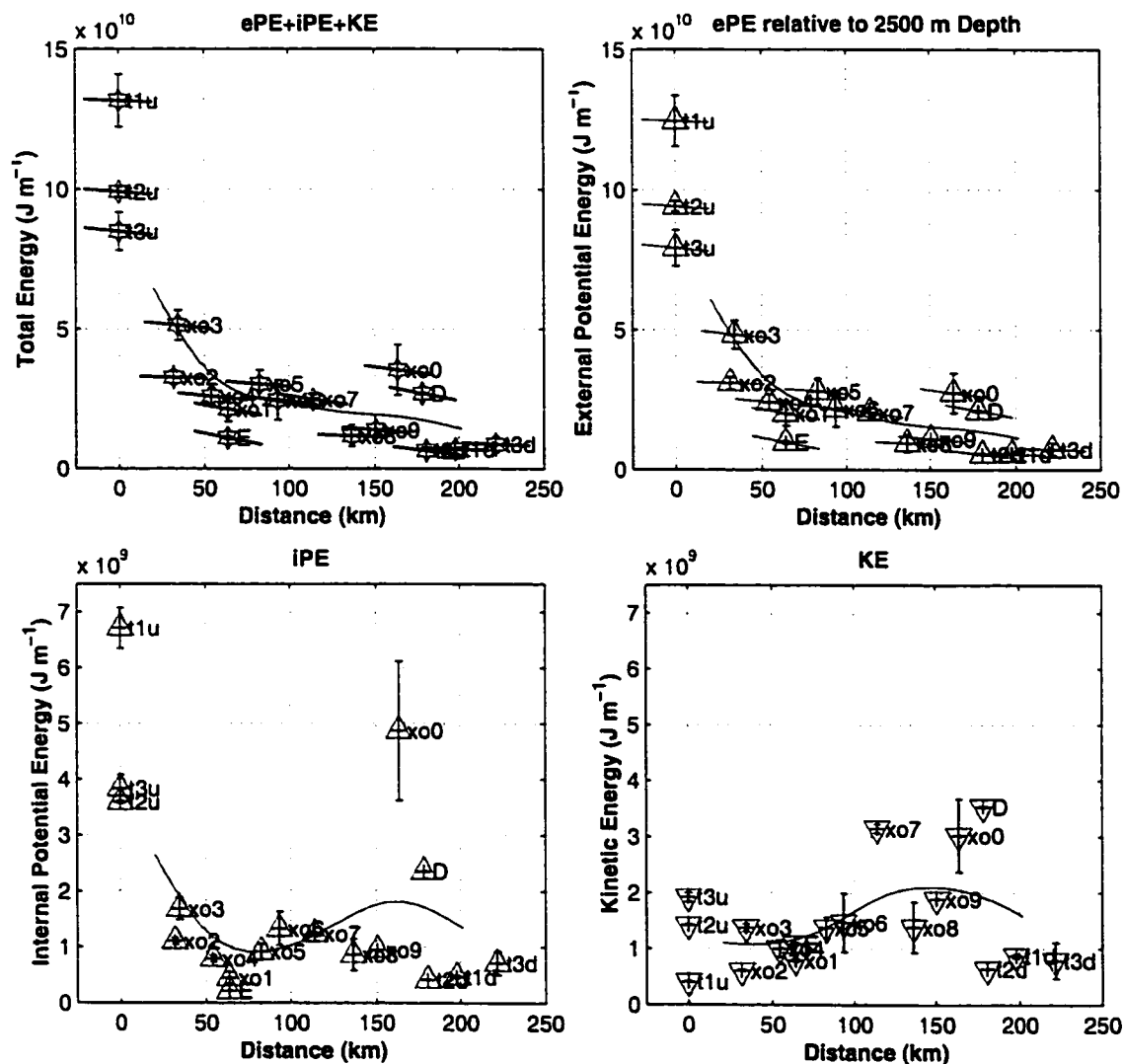
Figure 6.11: Evolution of energy terms with distance from the sill. Note the exponent in the y -axis, with the energy range of the upper two panels a factor of 20 greater than the lower two. The sloping lines on upper-left panel indicate rate of energy loss expected from bottom friction measurements at each section, as determined from Eq. 6.18 (and neglecting \tau_b ). Solid curves are the values smoothed with a 40 km Gaussian window.
