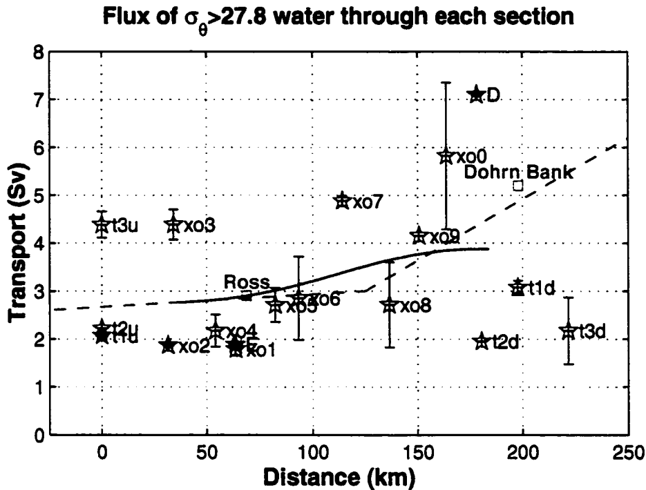
Figure 6.9: Dense water transport ( Q ) vs. distance from the sill, as measured by all 18 sections with XCPs (including two from the Aranda ) as well as two current meter arrays (labeled as “Ross” and “Dohrn Bank”). Green dashed lines show rates of transport increase expected from constant w_e values of 6 \times 10^{-5} \text{ m s}^{-1} and 8 \times 10^{-4} \text{ m s}^{-1} (estimated from Eq. 6.13 and Fig. 6.8 lines) over widths of 44 km and 32 km (average values of 2 \times H_{0.5} in the regions before and after 125 km, respectively). The red curve is from a smoothing of the Q values with a 75 km Gaussian filter.
