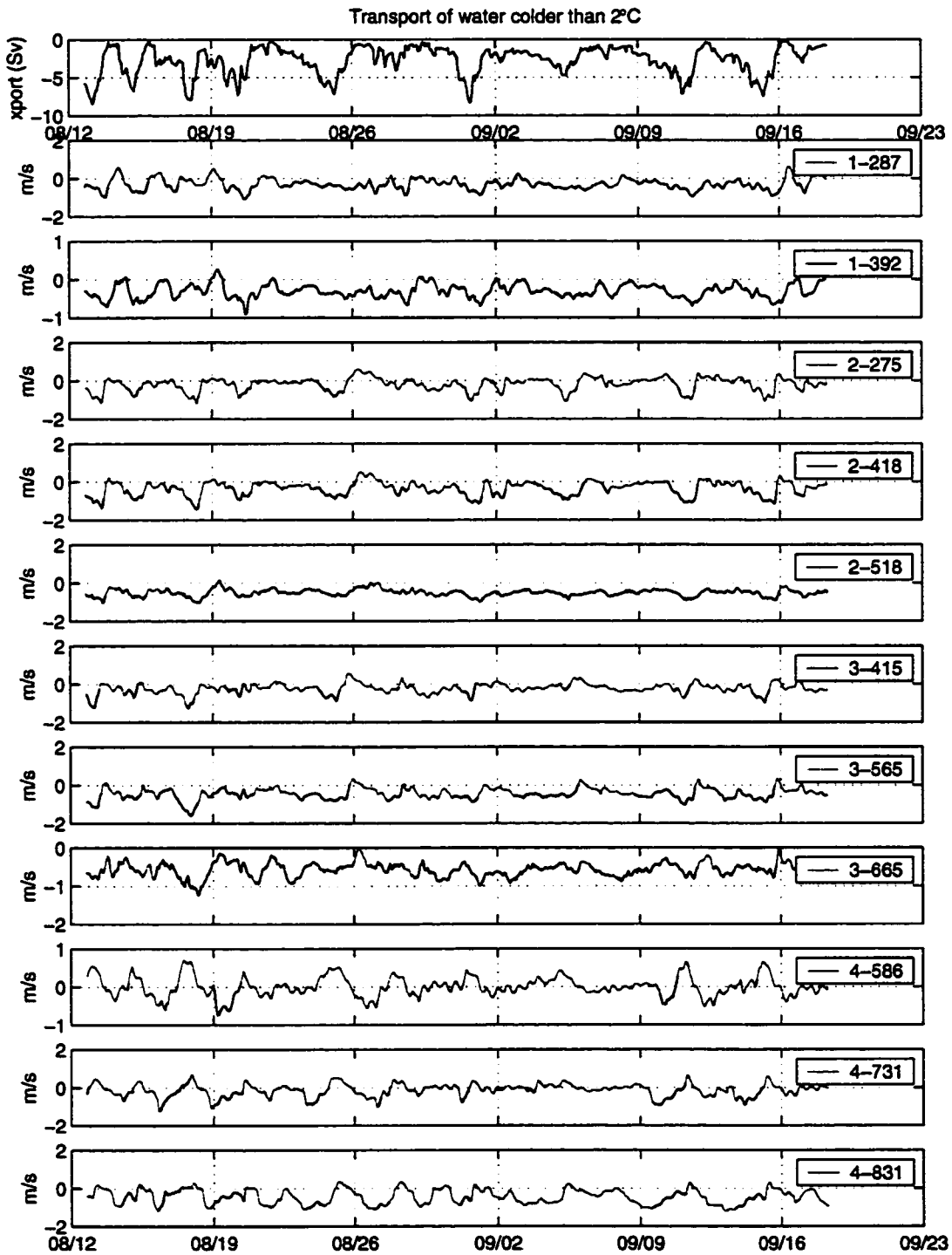
Figure 5.3: Top panel: Timeseries of transport of water colder than 2°C from O73 current meters. Negative values indicate flow to the southwest (towards 250°T). Other panels: Timeseries of velocity normal to the O73 array at each current meter. Blue indicates water colder than 2°C. Meters are labeled with the mooring number (1–4, where 1 is on the Greenland shelf) and instrument depth so that, e.g. , 4-831 is at 831 m depth on mooring 4.
