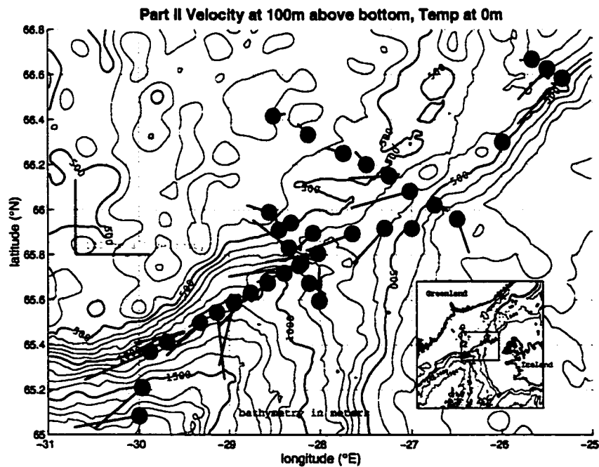
Figure 4.7: Same as Figure 4.5, Part II.
