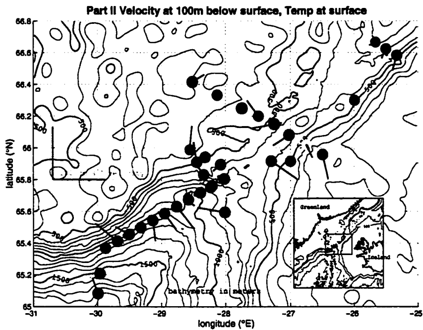
Figure 4.6: Same as Figure 4.4, Part II.
