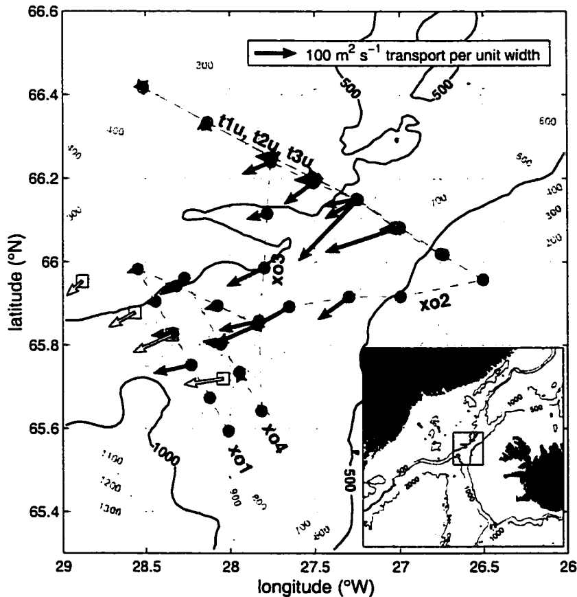
Figure 5.1: Locations of 1998 XCP/XCTD drops (dots) and 1973 current meters (squares). Open arrows are 5-week means of cold ( \theta < 2^\circ\text{C} ) water transport from the current meters. Solid arrows are dense ( \sigma_\theta > 27.8 ) water transport from single profiles. Bathymetry in meters from the Smith and Sandwell [1997] database is shown.
