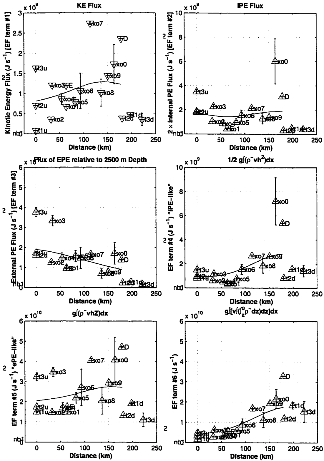
Figure 6.12: Through-section energy flux vs. downstream distance. Each panel shows one of the six terms in \iint_A (\mathbf{F}^{\text{tot}} \cdot \mathbf{j}) dz dx . Curves were smoothed with a 75 km Gaussian window.
