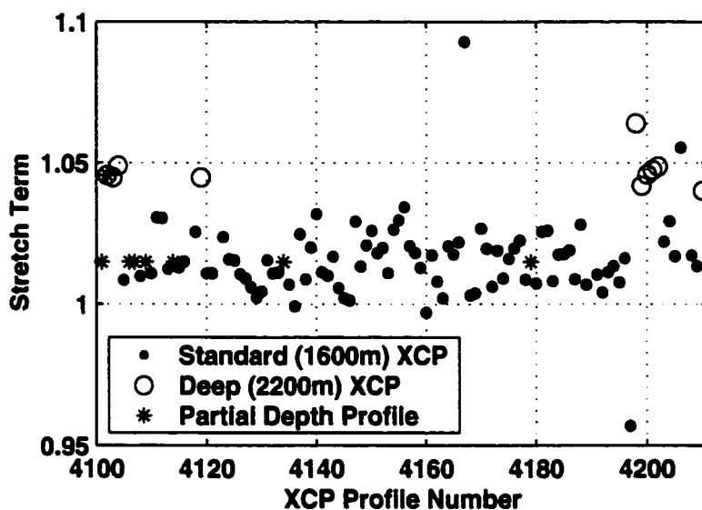
Figure 2.6: Linear stretching applied to the computed XCP profile depths, determined from comparison of XCP bottom hit with concurrently-measured corrected depth from the ES. Deep XCPs should require a systematically larger stretching term since they carry more wire and, hence, fall faster. Partial depth profiles are missing the top or bottom part of the profile, and so are stretched by an average value determined from other probes of the same type. The scatter is most likely due to inter-probe differences, but variability in the ES correction (see Section 2.1.1) plays some role.
