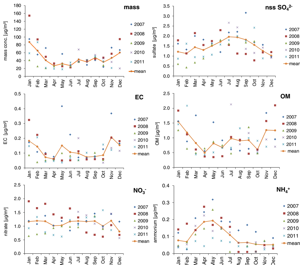
Figure 4. Annual variability and monthly mean of \text{PM}_{10} mass concentration, non-sea-salt sulfate, elemental carbon (EC), organic matter (OM), nitrate and ammonium during the 5 years of measurements for samples collected on the tower.
